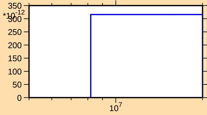
\sigma vs. E for ^{197}\text{Po}(n,\text{pt})
