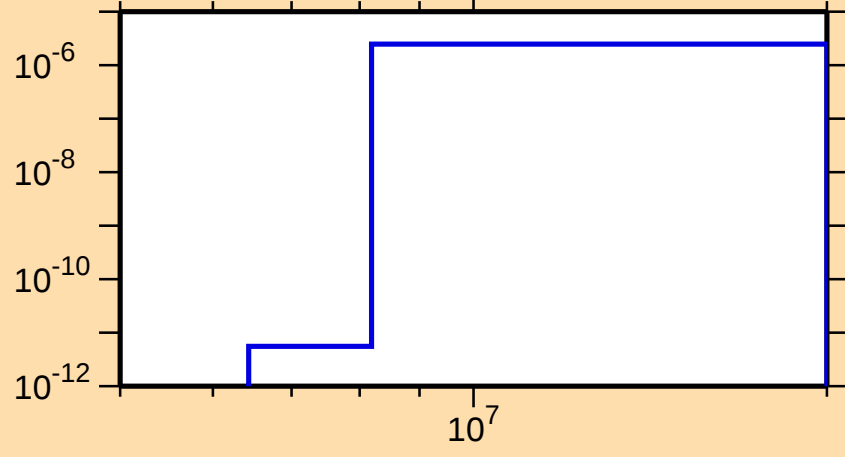
\sigma vs. E for ^{197}\text{Po}(n,\text{He}3)
