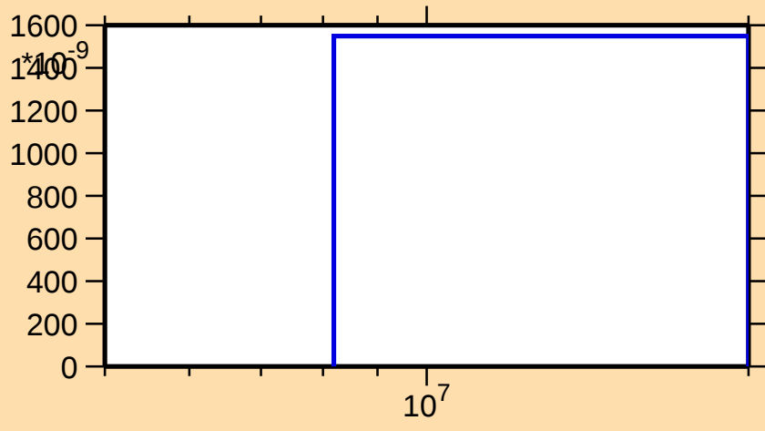
\sigma vs. E for ^{197}\text{Po}(n,2np)
