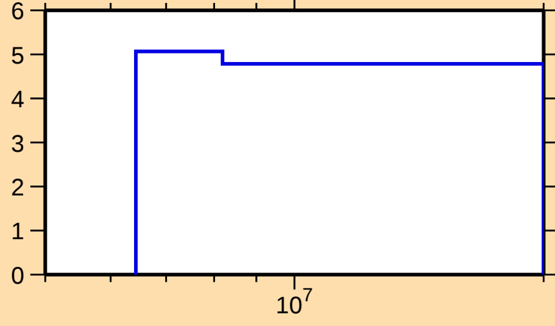
\Delta\sigma/\sigma vs. E for ^{197}\text{Po}(n,\text{nonel.})
