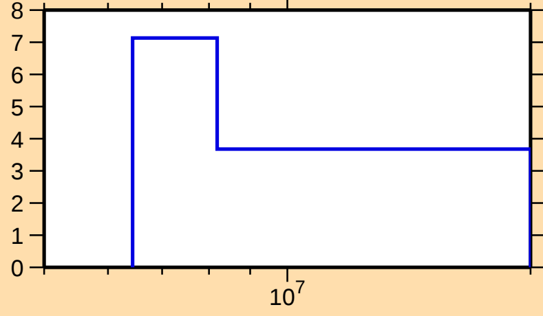
\Delta\sigma/\sigma vs. E for ^{197}\text{Po}(n,\text{tot.})
