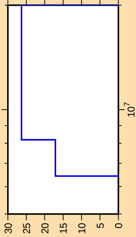
\Delta\sigma/\sigma vs. E for ^{197}\text{Po}(n,n\text{cont.})
