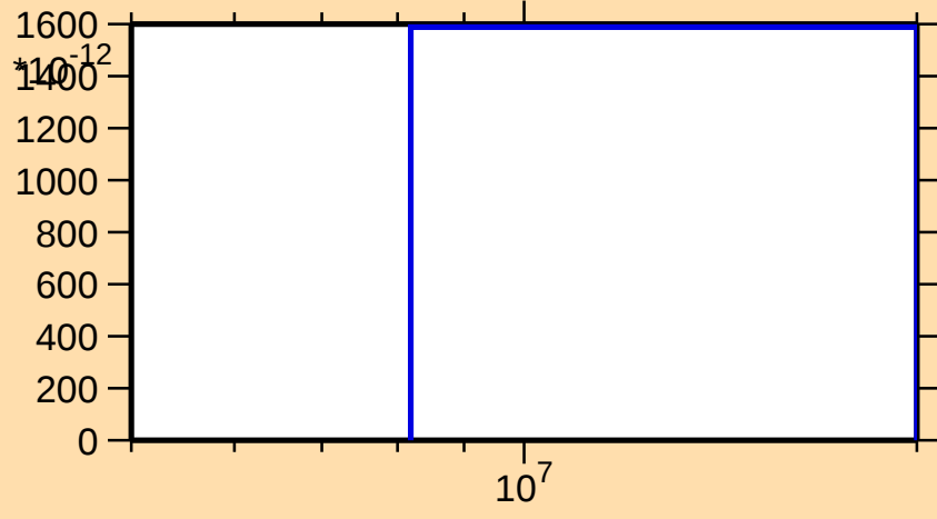
\sigma vs. E for ^{197}\text{Po}(\text{mt } 45)
