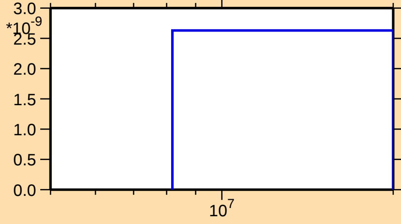
\sigma vs. E for ^{197}\text{Po}(n,\text{pd})
