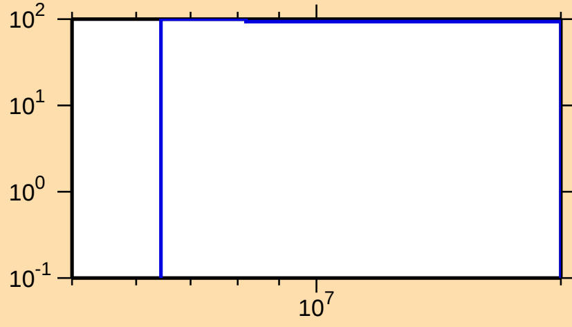
\Delta\sigma/\sigma vs. E for ^{197}\text{Po}(n,2n)
