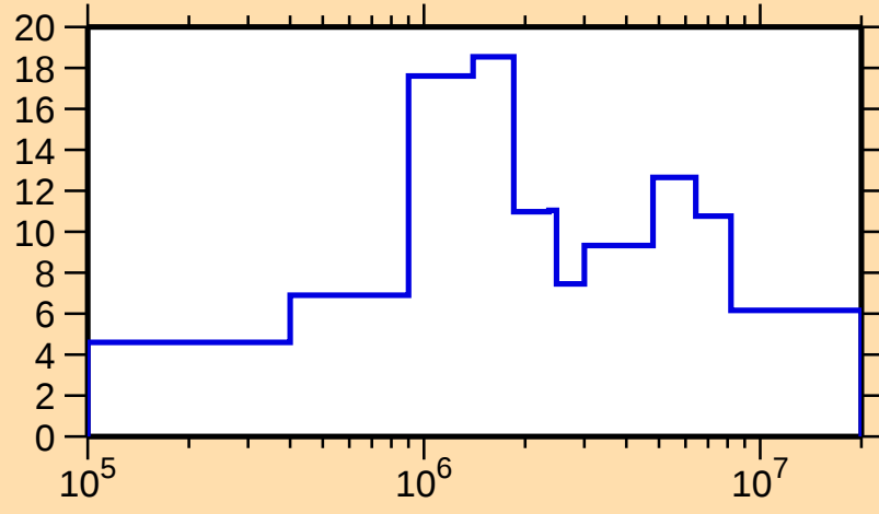
\Delta\sigma/\sigma vs. E for ^{197}\text{Po}(n,\text{el.})
