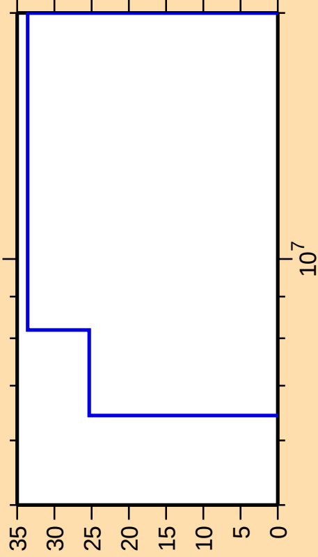
\Delta\sigma/\sigma vs. E for ^{197}\text{Po}(n,n_1)
