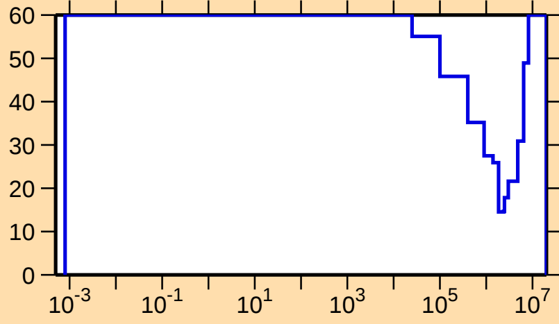
\Delta\sigma/\sigma vs. E for ^{197}\text{Po}(n,\gamma)
