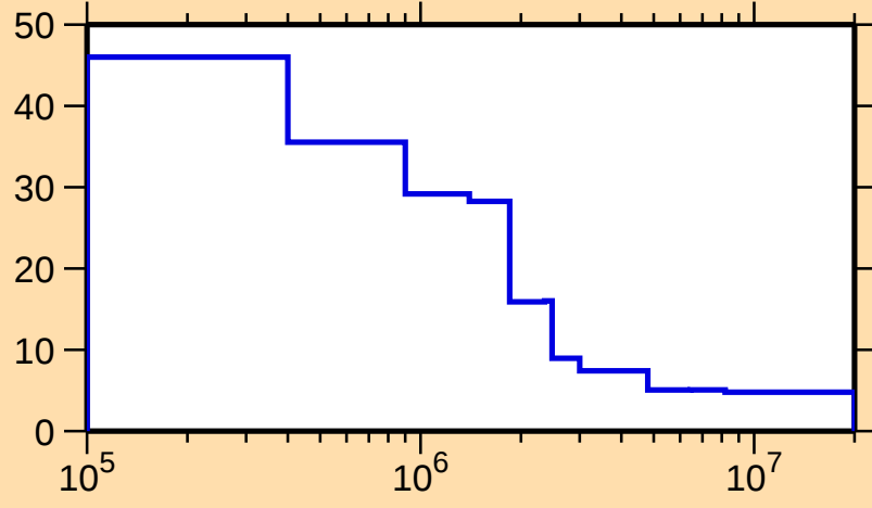
\Delta\sigma/\sigma vs. E for ^{197}\text{Po}(\text{n},\text{nonel.})
