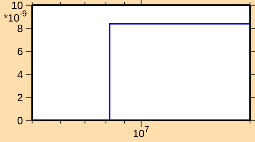
\sigma vs. E for ^{197}\text{Po}(n,\text{nd})
