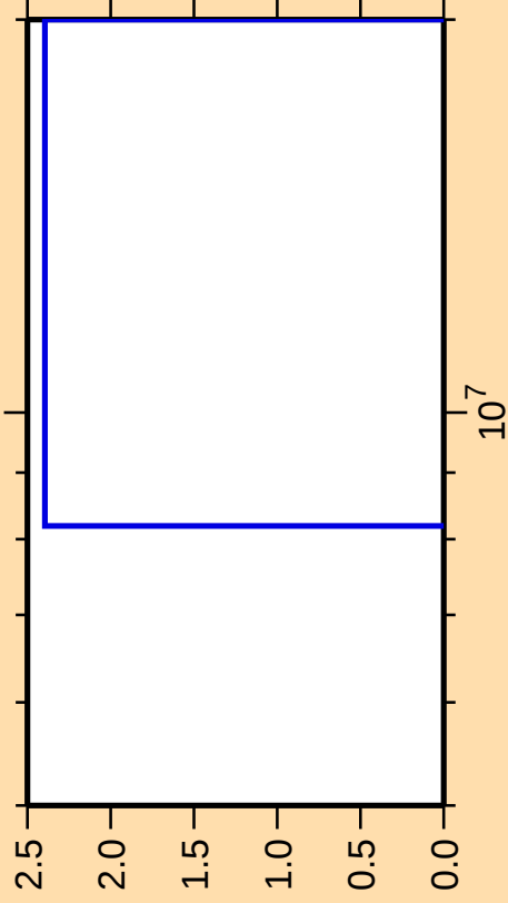
\Delta\sigma/\sigma vs. E for ^{197}\text{Po}(n,nt)
