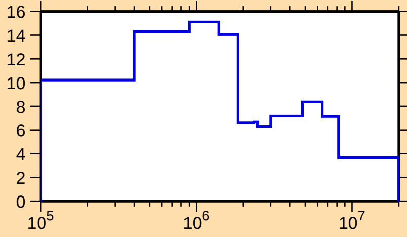
\Delta\sigma/\sigma vs. E for ^{197}\text{Po}(n,\text{tot.})
