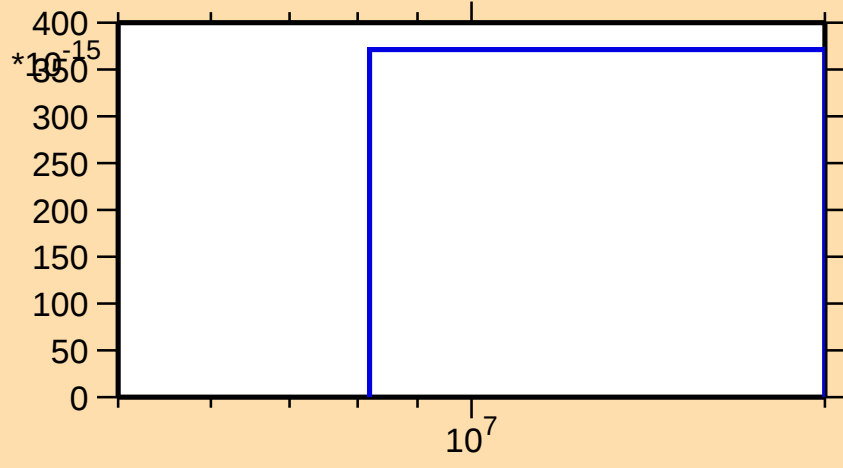
\sigma vs. E for ^{197}\text{Po}(n,nt)
