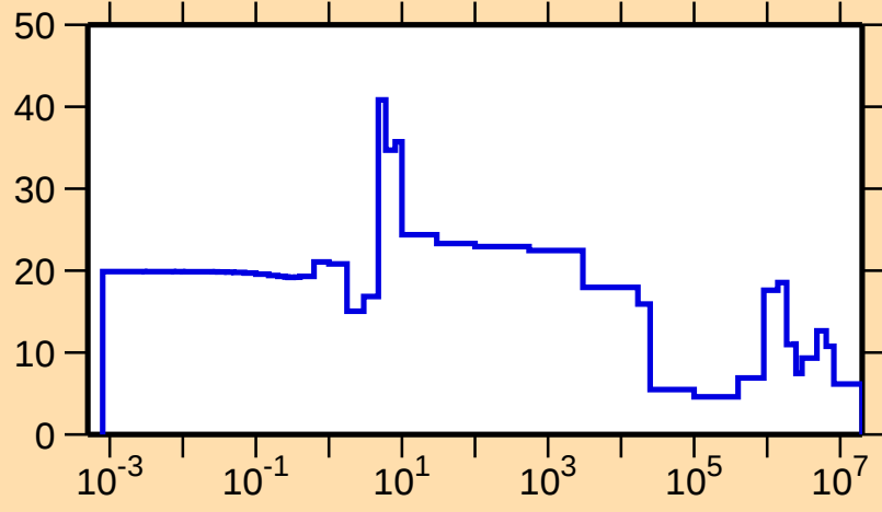
\Delta\sigma/\sigma vs. E for ^{197}\text{Po}(n,\text{el.})
