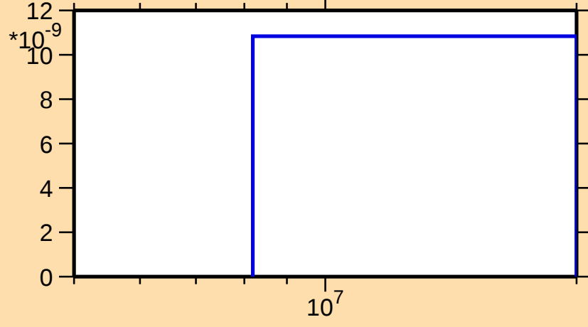
\sigma vs. E for ^{197}\text{Po}(n,3n)
