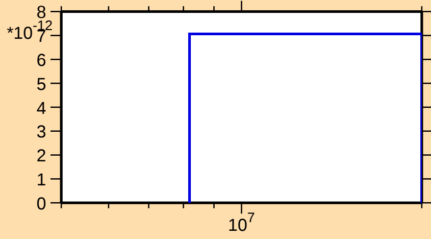
\sigma vs. E for ^{197}\text{Po}(\text{mt } 34)
