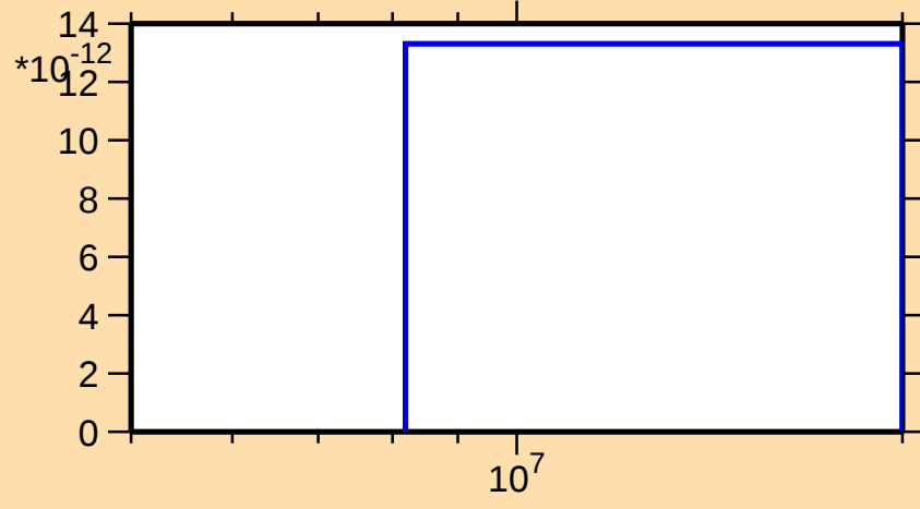
\sigma vs. E for ^{197}\text{Po}(\text{mt117})
