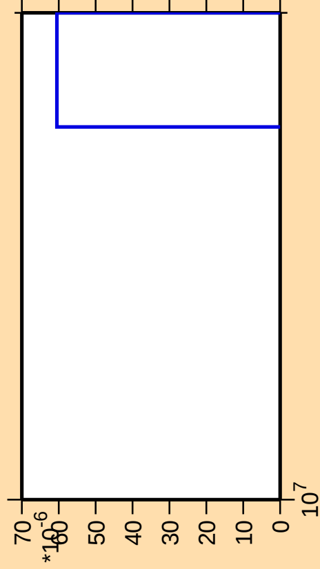
\Delta\sigma/\sigma vs. E for ^{198}\text{Po}(\text{mt 11})
