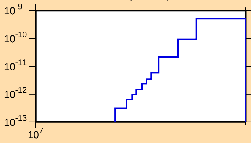
\sigma vs. E for ^{198}\text{Po}(\text{mt117})
