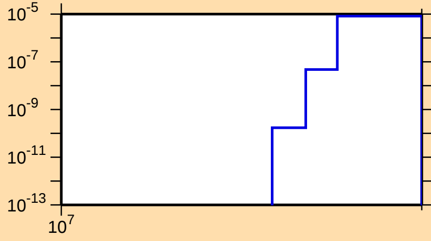
\sigma vs. E for ^{198}\text{Po}(n,2np)
