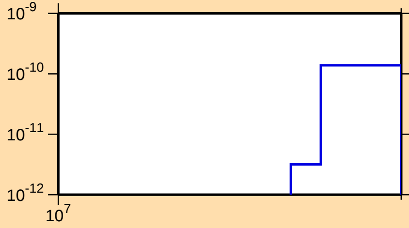
\sigma vs. E for ^{198}\text{Po}(n,\text{pt})
