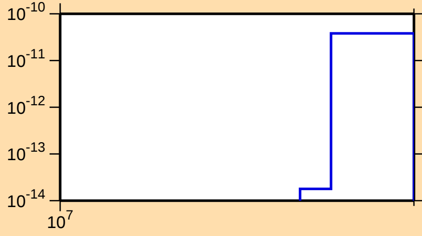
\sigma vs. E for ^{198}\text{Po}(n,nt)
