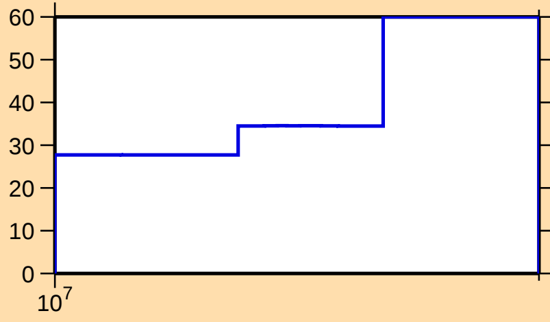
\Delta\sigma/\sigma vs. E for ^{198}\text{Po}(n,\text{inel.})
