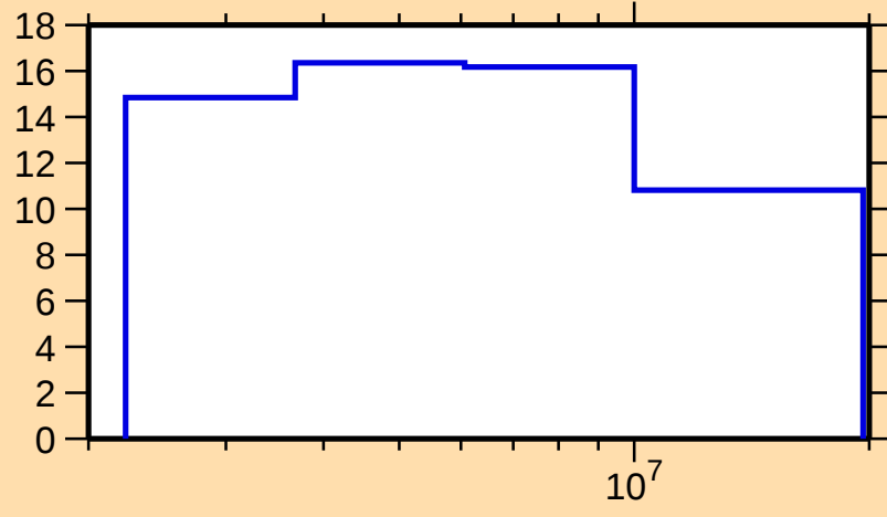
\Delta\sigma/\sigma vs. E for ^{198}\text{Po}(n,\text{tot.})
