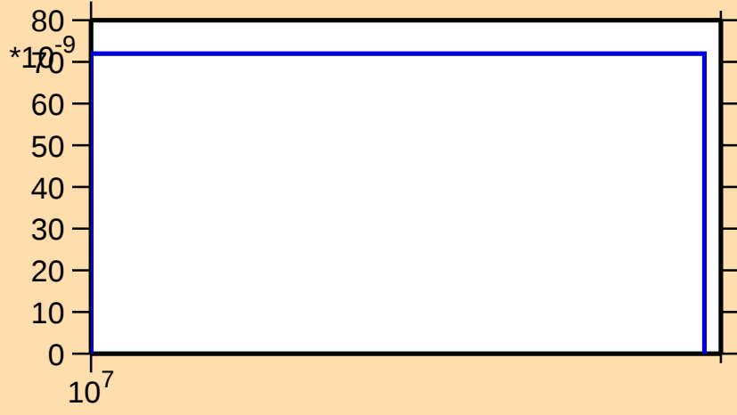
\sigma vs. E for ^{198}\text{Po}(n,2np)
