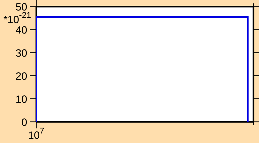
\sigma vs. E for ^{198}\text{Po}(\text{mt } 11)
