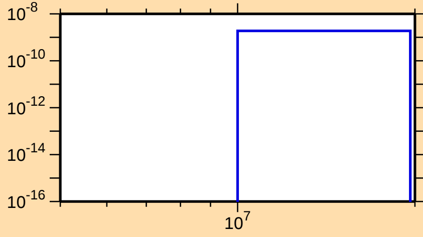
\sigma vs. E for ^{198}\text{Po}(n,\text{pd})
