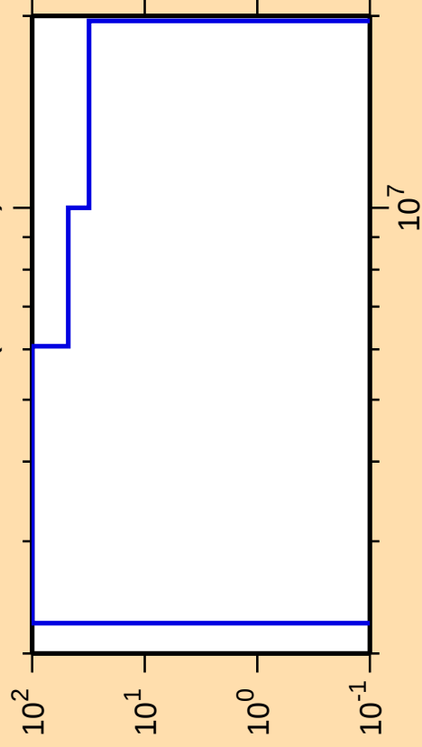
\Delta\sigma/\sigma vs. E for ^{198}\text{Po}(n,n_{\text{cont}})
