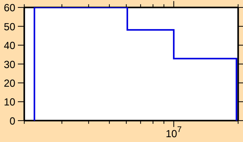
\Delta\sigma/\sigma vs. E for ^{198}\text{Po}(\text{n},\text{inel.})
