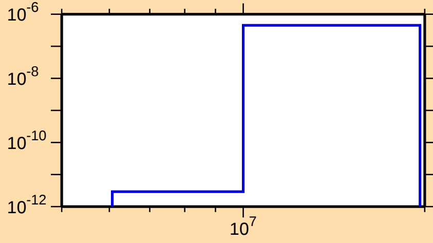
\sigma vs. E for ^{198}\text{Po}(n,\text{He}3)
