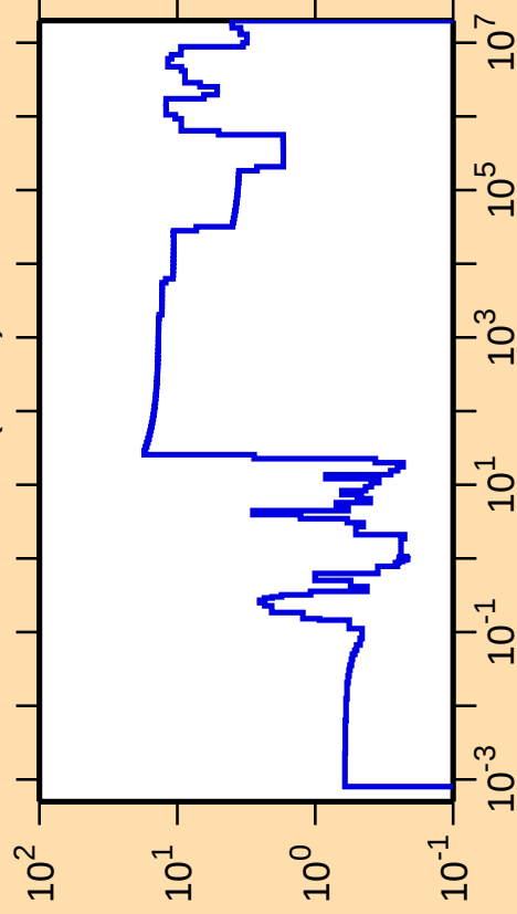
\Delta\sigma/\sigma vs. E for ^{199}\text{Po}(\text{n},\text{el.})
