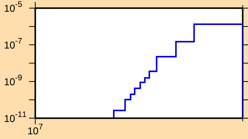
\sigma vs. E for ^{199}\text{Po}(n,\text{nd})
