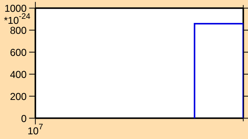
\sigma vs. E for ^{199}\text{Po}(\text{mt } 11)
