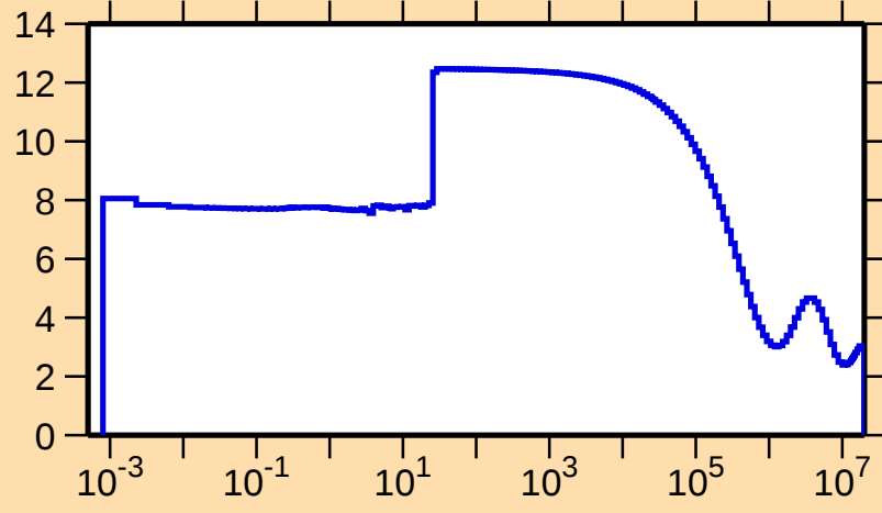
\sigma vs. E for ^{199}\text{Po}(\text{n},\text{el.})
