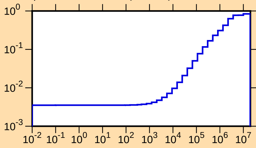
\mu vs. E for ^{199}\text{Po}(\text{mt251})
