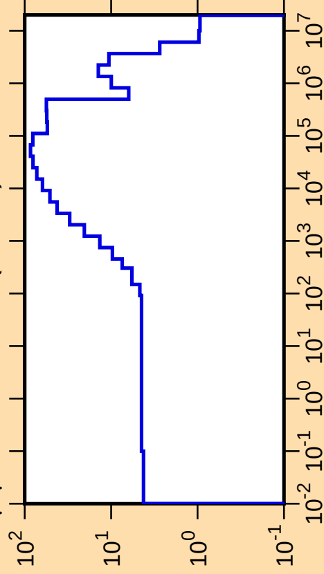
\Delta\mu/\mu vs. E for ^{199}\text{Po}(\text{mt251})
