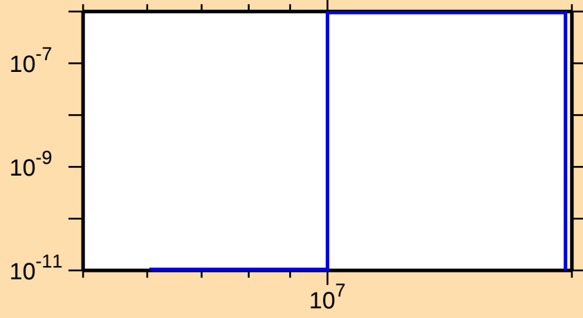
\sigma vs. E for ^{199}\text{Po}(n,\text{He}3)
