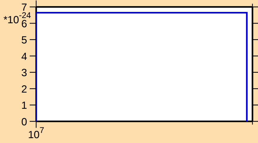
\sigma vs. E for ^{199}\text{Po}(\text{mt 11})
