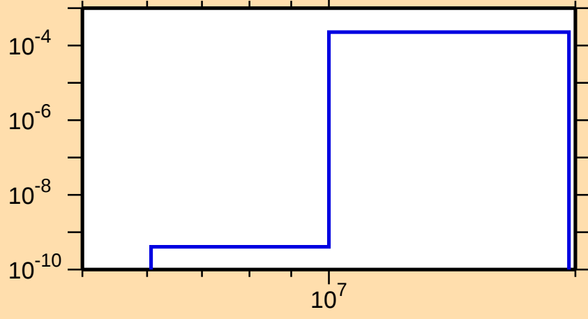
\sigma vs. E for ^{199}\text{Po}(n,t)
