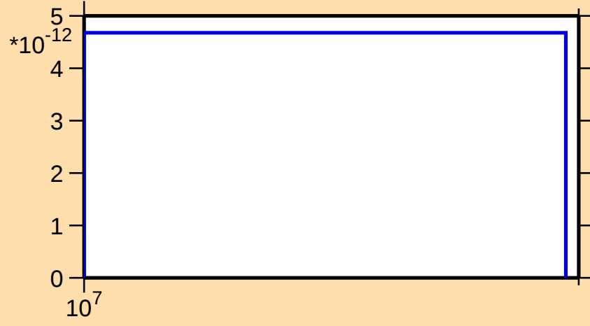
\sigma vs. E for ^{199}\text{Po}(\text{mt } 34)
