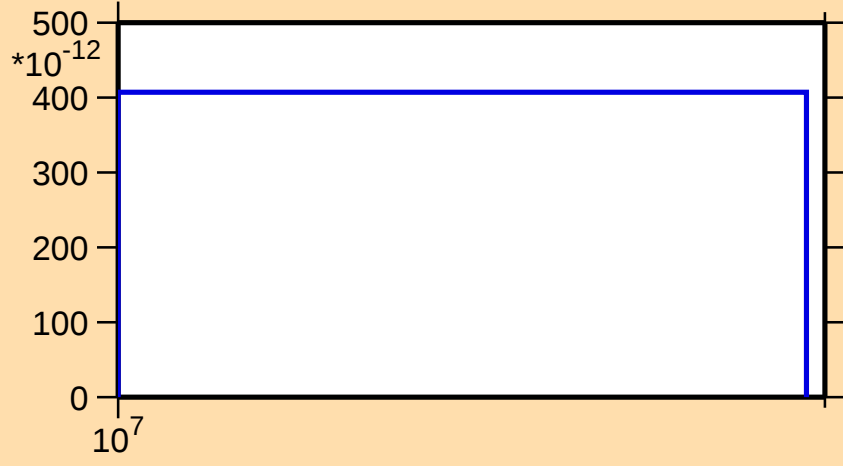
\sigma vs. E for ^{199}\text{Po}(\text{mt } 45)
