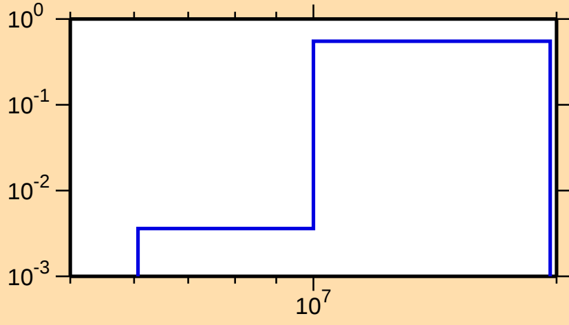
\sigma vs. E for ^{199}\text{Po}(n,2n)
