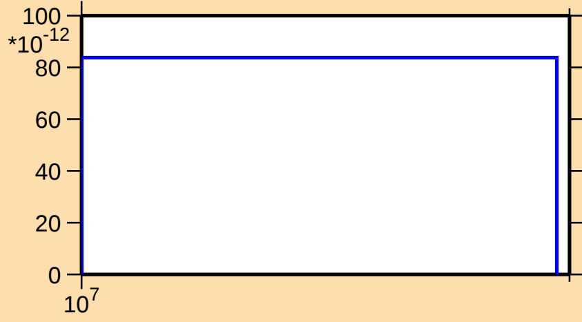
\sigma vs. E for ^{199}\text{Po}(n,\text{pt})
