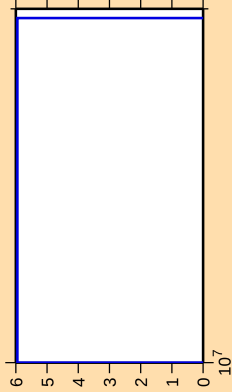
\Delta\sigma/\sigma vs. E for ^{199}\text{Po}(n,nt)
