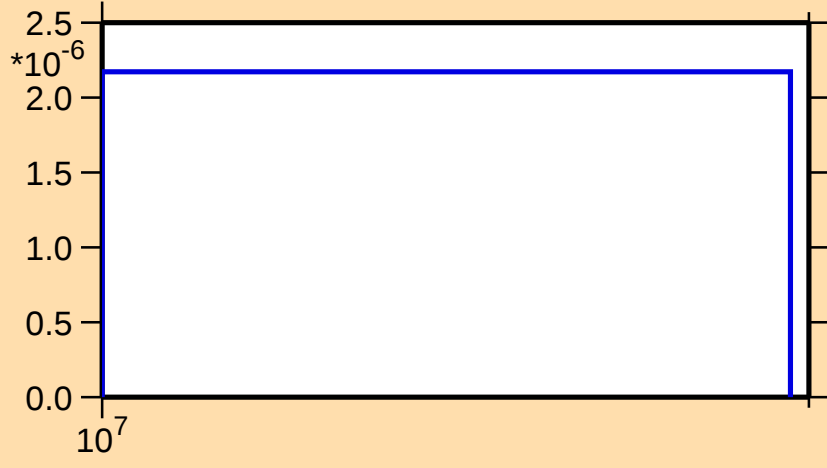
\sigma vs. E for ^{199}\text{Po}(n,2np)
