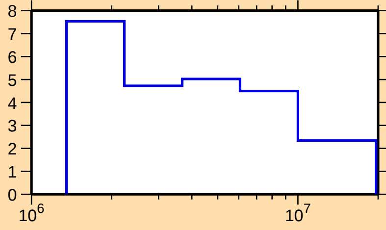
\Delta\sigma/\sigma vs. E for ^{199}\text{Po}(n,\text{tot.})
