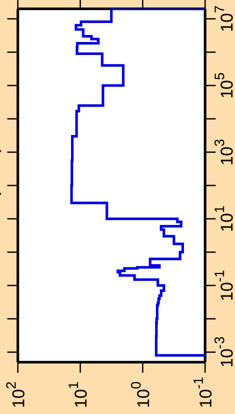
\Delta\sigma/\sigma vs. E for ^{199}\text{Po}(n,\text{el.})
