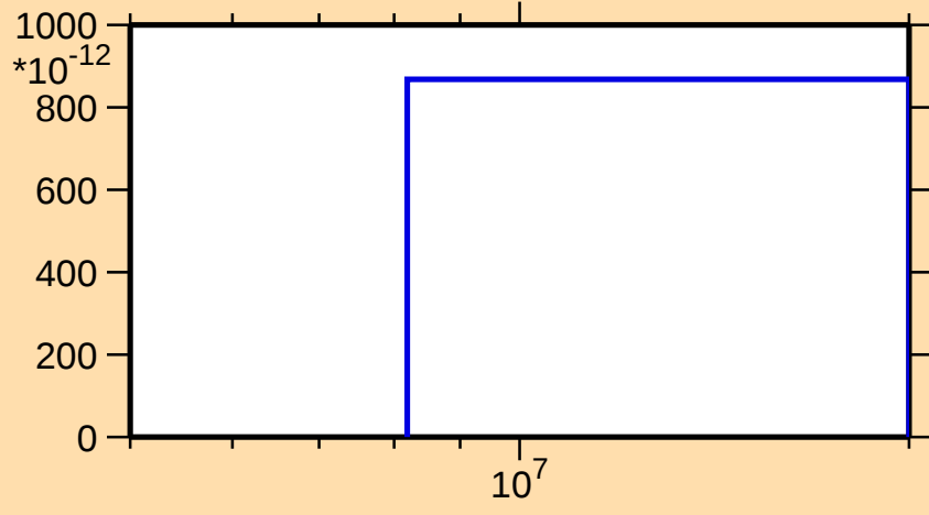
\sigma vs. E for ^{199}\text{Po}(n,\text{pd})
