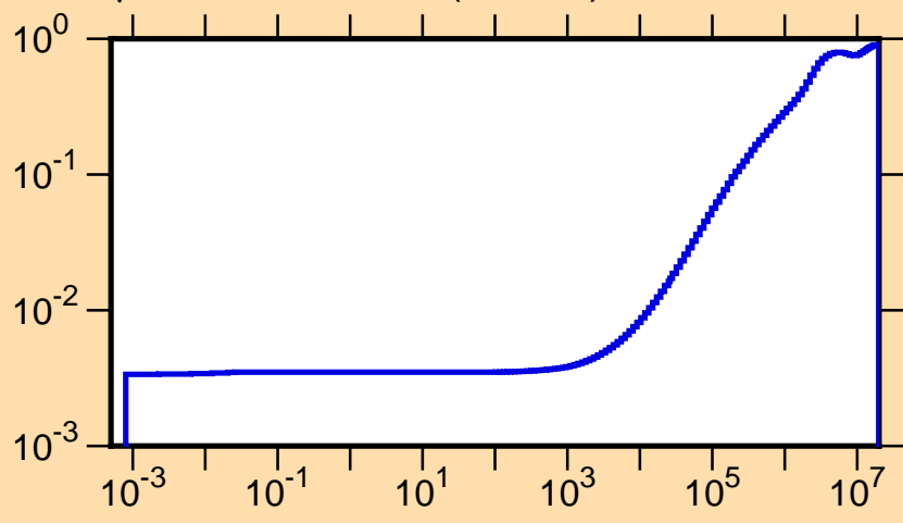
\mu vs. E for ^{200}\text{Po}(\text{mt251})
