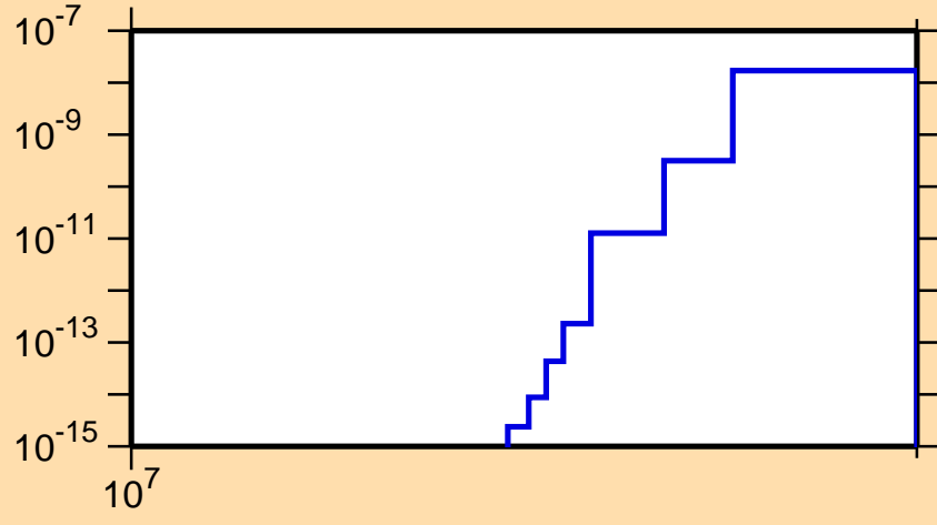
\sigma vs. E for ^{200}\text{Po}(n,\text{nd})
