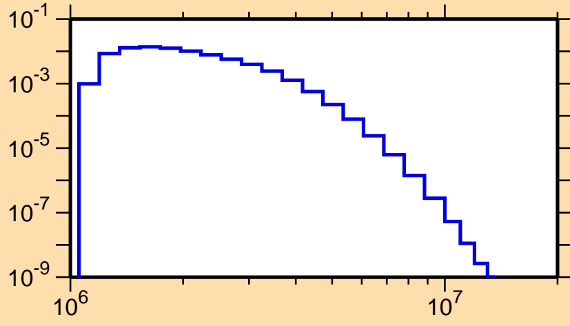
\sigma vs. E for ^{200}\text{Po}(n,n_2)
