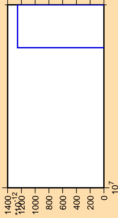
\Delta\sigma/\sigma vs. E for ^{200}\text{Po}(\text{mt 11})
