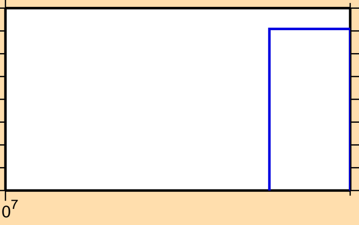
\sigma vs. E for ^{200}\text{Po}(n,3n)
