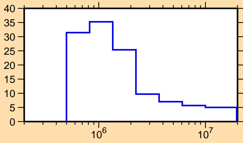
\Delta\sigma/\sigma vs. E for ^{200}\text{Po}(n,\text{nonel.})
