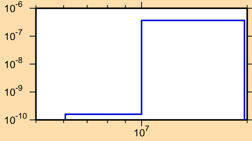
\sigma vs. E for ^{200}\text{Po}(n,p\alpha)
