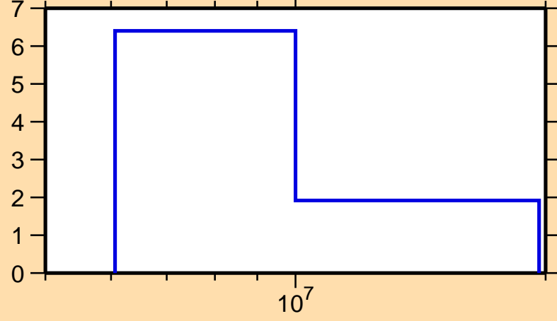
\Delta\sigma/\sigma vs. E for ^{200}\text{Po}(n,\text{tot.})
