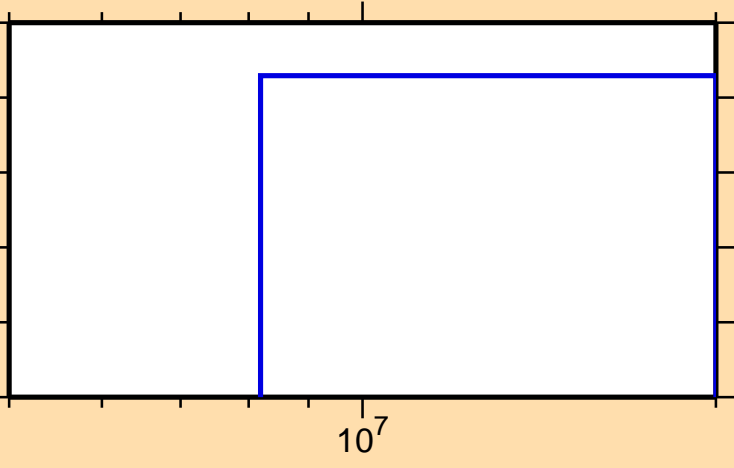
\sigma vs. E for ^{200}\text{Po}(n,t)
