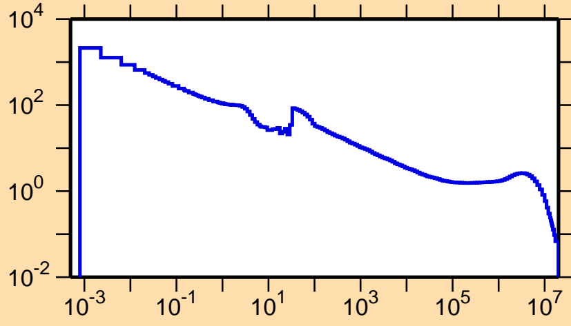
\sigma vs. E for ^{201}\text{Po}(n,\gamma)
