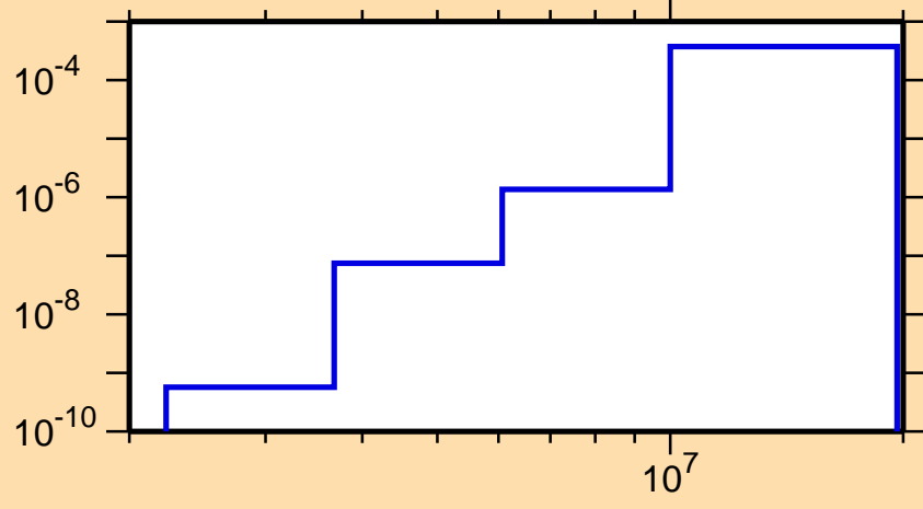
\sigma vs. E for ^{201}\text{Po}(n,n\alpha)
