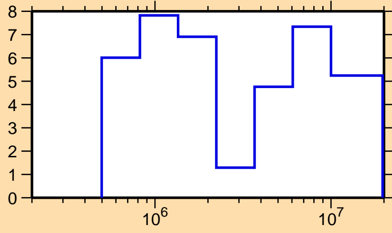
\Delta\sigma/\sigma vs. E for ^{201}\text{Po}(n,\text{el.})
