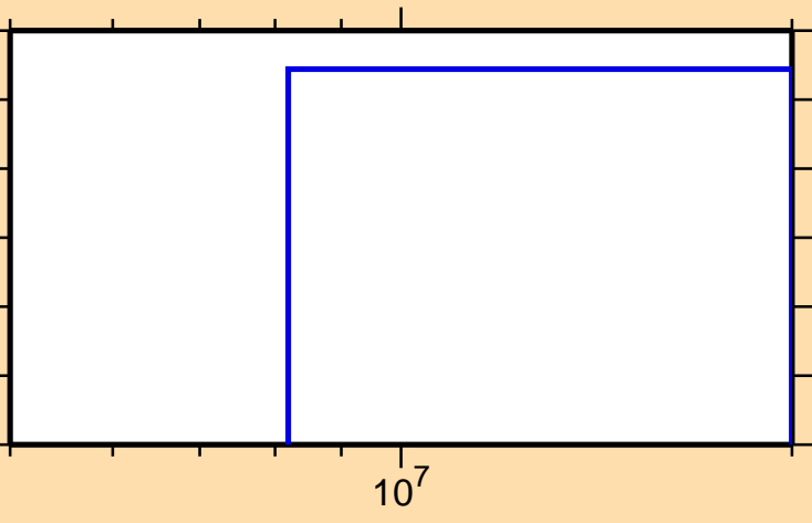
\sigma vs. E for ^{201}\text{Po}(n,\text{nd})
