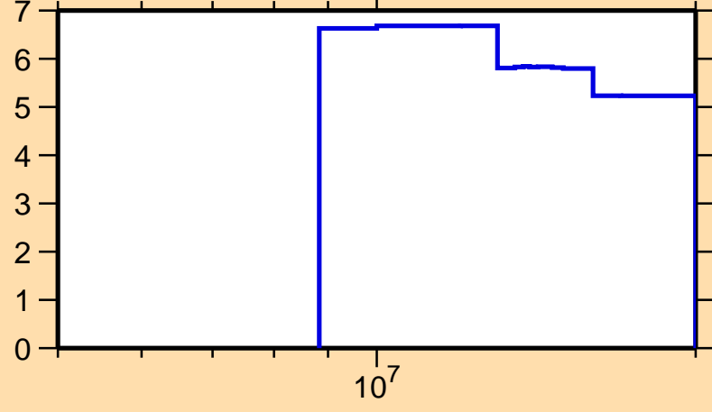
\Delta\sigma/\sigma vs. E for ^{202}\text{Po}(n,\text{nonel.})
