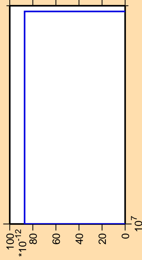
\Delta\sigma/\sigma vs. E for ^{202}\text{Po} (mt 11)
