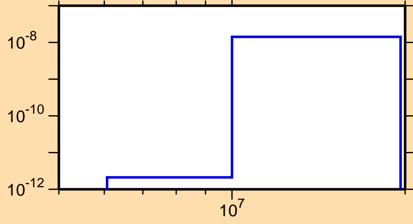
\sigma vs. E for ^{202}\text{Po}(n,p\alpha)
