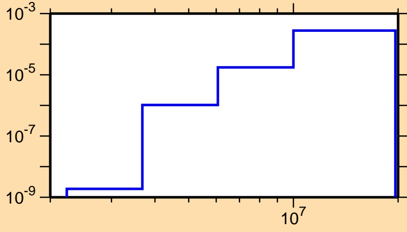
\sigma vs. E for ^{202}\text{Po}(n,n\alpha)
