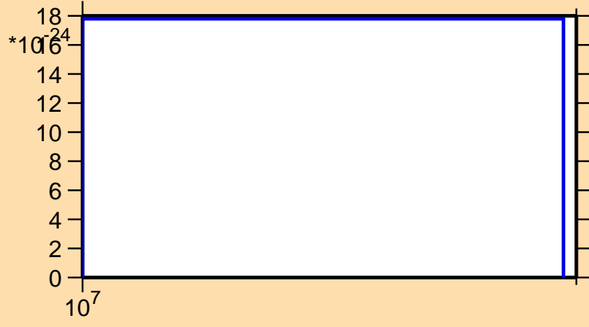
\sigma vs. E for ^{202}\text{Po} (mt 11)
