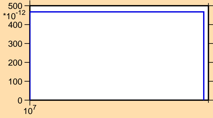
\sigma vs. E for ^{202}\text{Po}(n,\text{nd})
