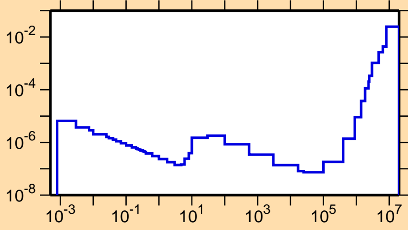
\sigma vs. E for ^{202}\text{Po}(n,p)
