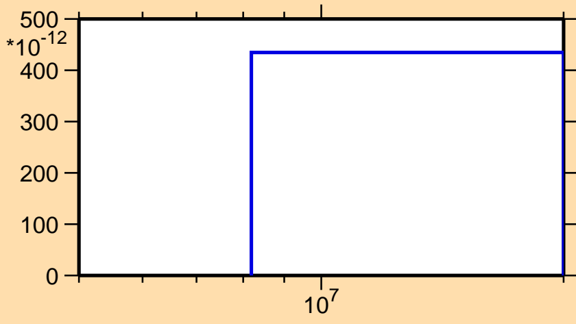
\sigma vs. E for ^{202}\text{Po}(n,\text{nd})
