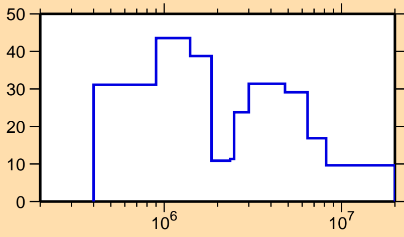
\Delta\sigma/\sigma vs. E for ^{202}\text{Po}(n,\text{el.})
