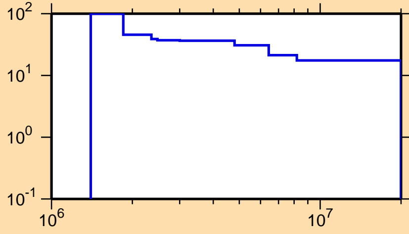
\Delta\sigma/\sigma vs. E for ^{202}\text{Po}(n, n\text{cont.})
