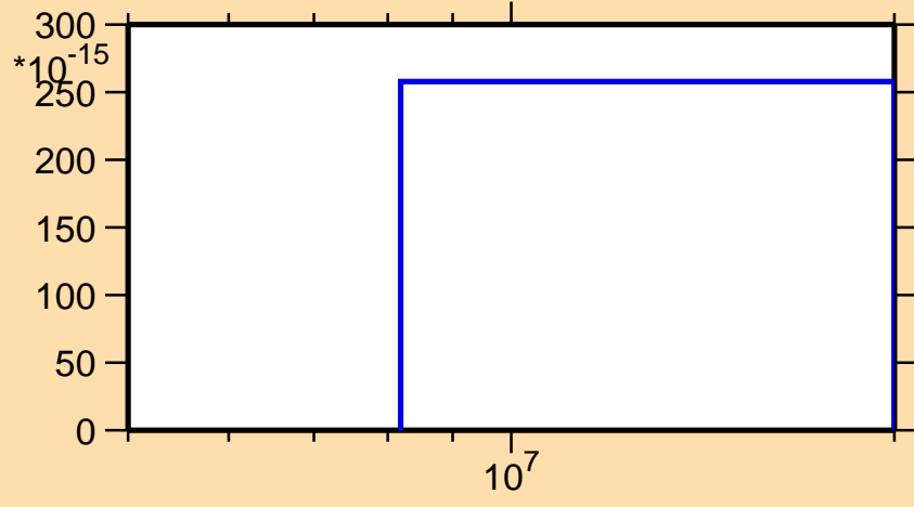
\sigma vs. E for ^{202}\text{Po}(n,\text{pt})
