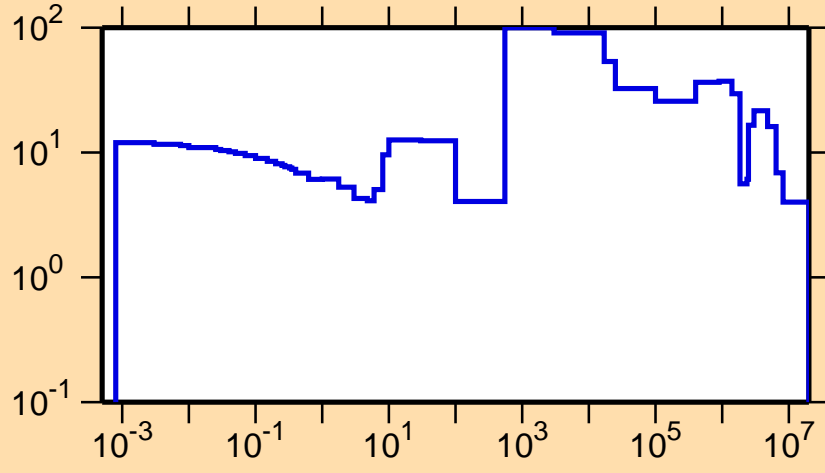
\Delta\sigma/\sigma vs. E for ^{202}\text{Po}(n,\text{tot.})
