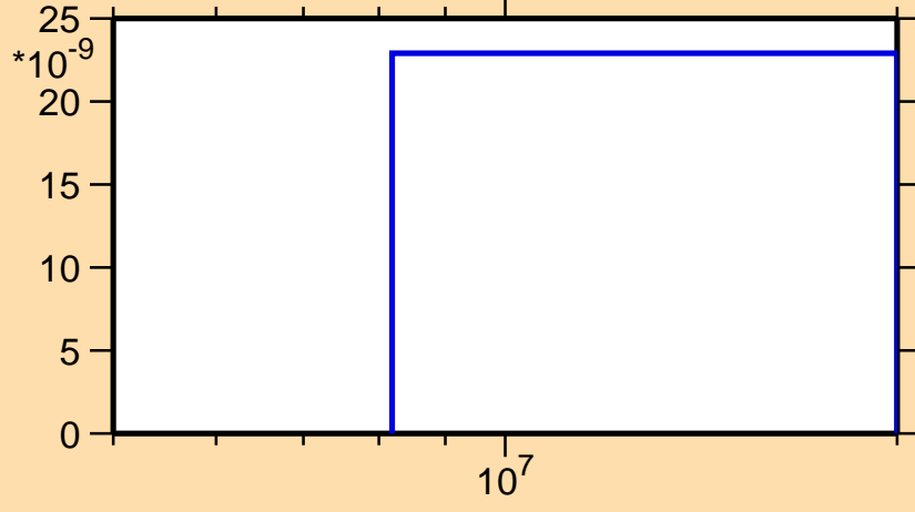
\sigma vs. E for ^{202}\text{Po}(n,\text{He}3)
