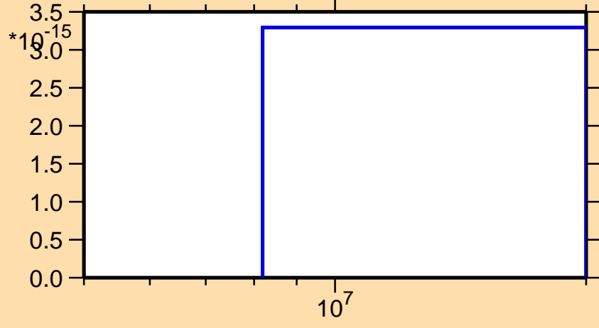
\sigma vs. E for ^{202}\text{Po}(n,3n\alpha)
