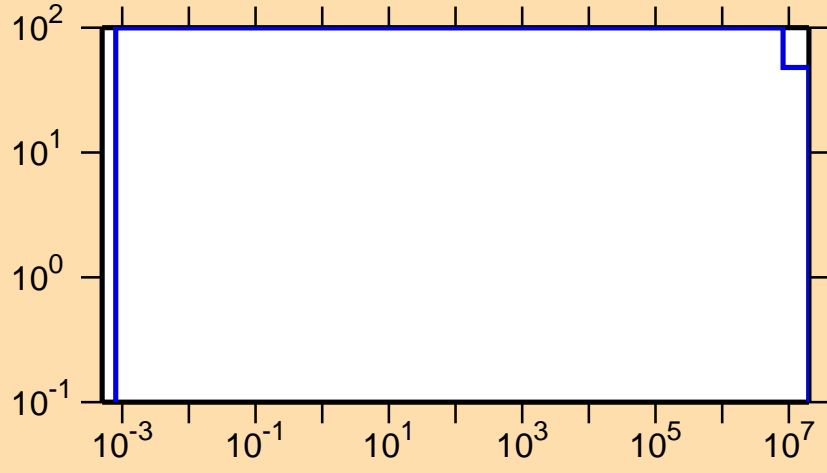
\Delta\sigma/\sigma vs. E for ^{202}\text{Po}(n,p)
