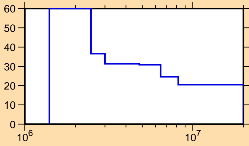
\Delta\sigma/\sigma vs. E for ^{202}\text{Po}(n,\text{inel.})
