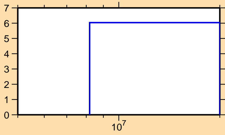
\Delta\sigma/\sigma vs. E for ^{202}\text{Po}(n,\text{nonel.})
