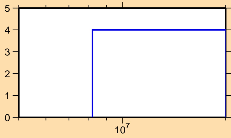
\Delta\sigma/\sigma vs. E for ^{202}\text{Po}(n,\text{tot.})
