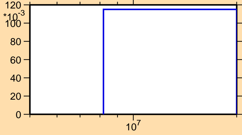
\sigma vs. E for ^{202}\text{Po}(n,2n)
