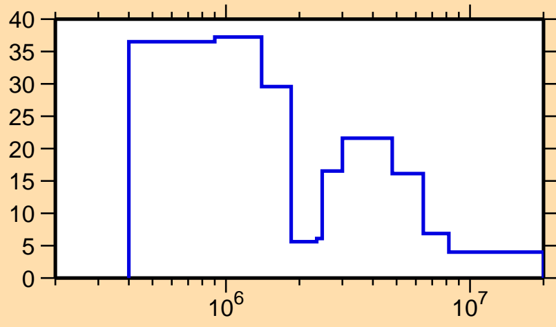
\Delta\sigma/\sigma vs. E for ^{202}\text{Po}(n,\text{tot.})
