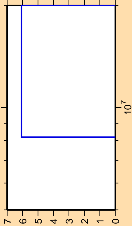
\Delta\sigma/\sigma vs. E for ^{202}\text{Po}(n,nt)
