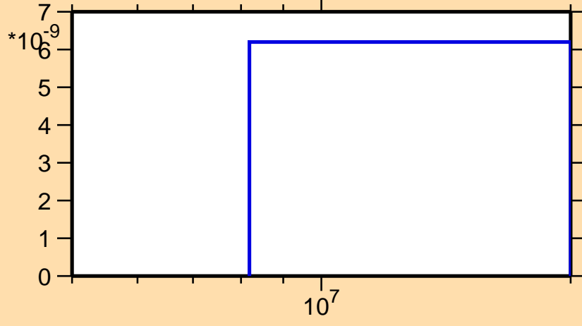
\sigma vs. E for ^{202}\text{Po}(n,2n\alpha)
