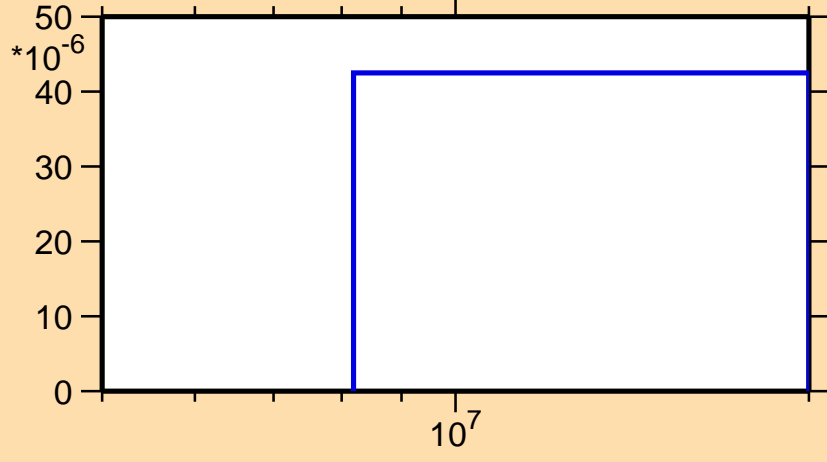
\sigma vs. E for ^{202}\text{Po}(n,t)
