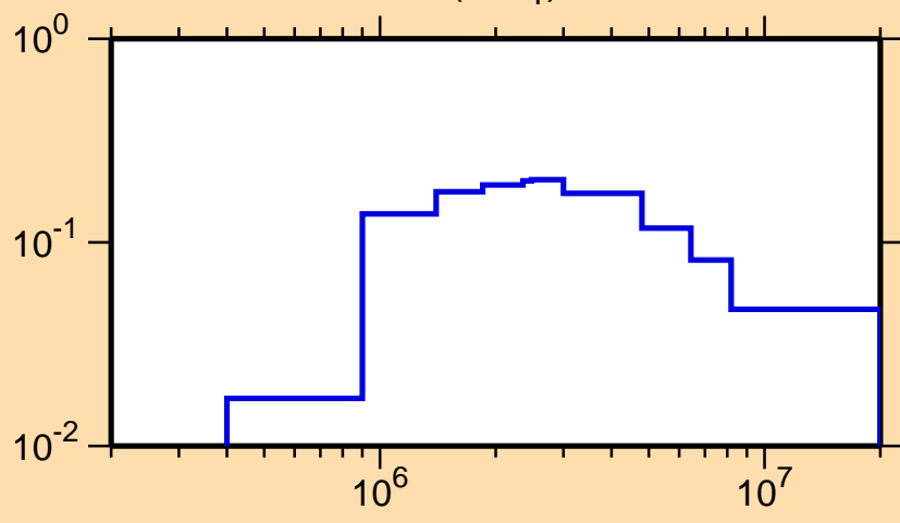
\sigma vs. E for ^{202}\text{Po}(n,n_1)
