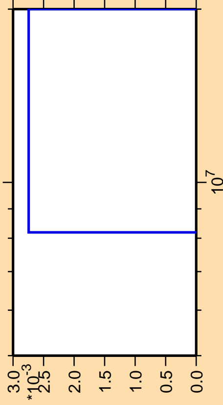
\Delta\sigma/\sigma vs. E for ^{202}\text{Po}(n,3n\alpha)
