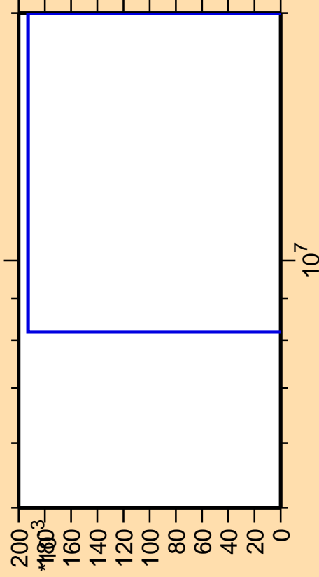
\Delta\sigma/\sigma vs. E for ^{202}\text{Po}(n,\text{pt})
