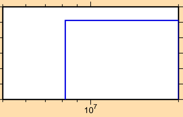
\sigma vs. E for ^{202}\text{Po}(n,2np)
