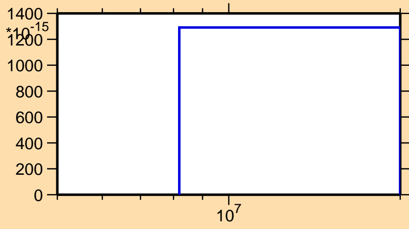
\sigma vs. E for ^{202}\text{Po}(n,nt)
