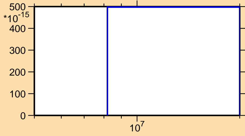
\sigma vs. E for ^{202}\text{Po} (mt 45)
