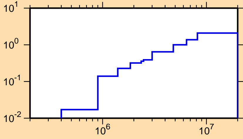
\sigma vs. E for ^{202}\text{Po}(n,\text{inel.})
