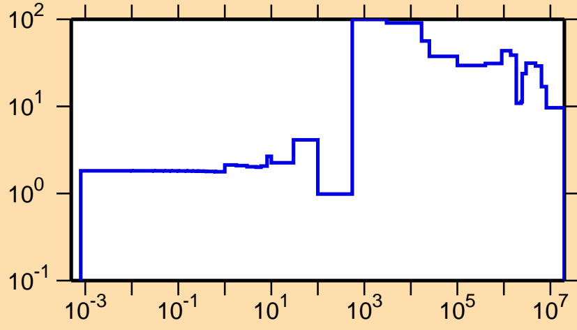
\Delta\sigma/\sigma vs. E for ^{202}\text{Po}(n,\text{el.})
