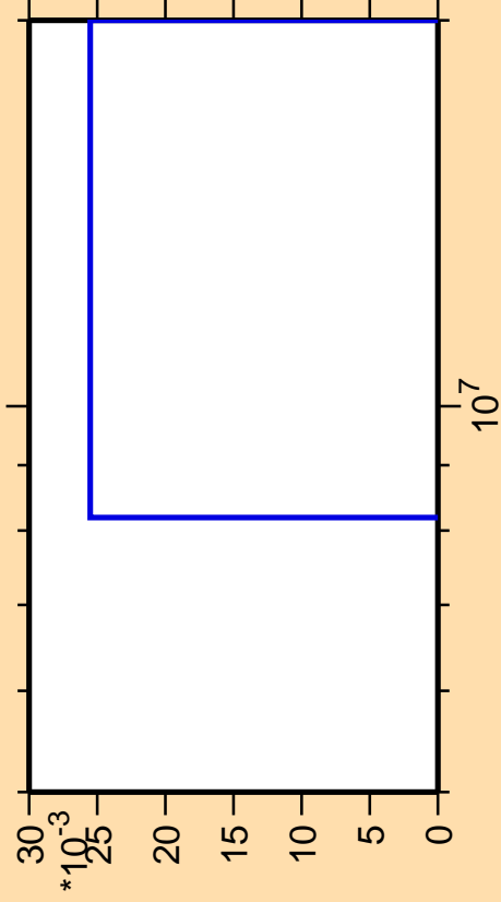
\Delta\sigma/\sigma vs. E for ^{202}\text{Po}(\text{mt117})
