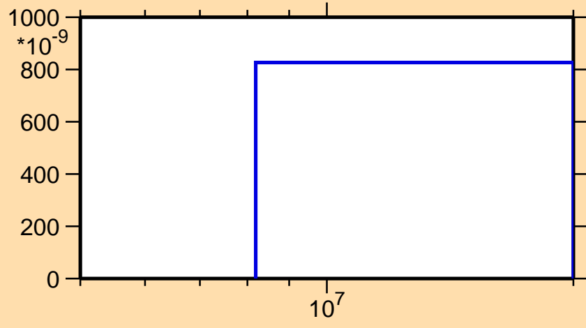
\sigma vs. E for ^{202}\text{Po}(n,3n)
