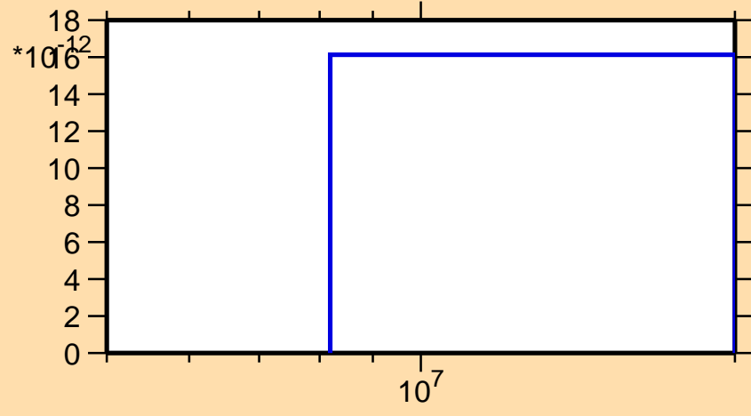
\sigma vs. E for ^{202}\text{Po}(n,\text{pd})
