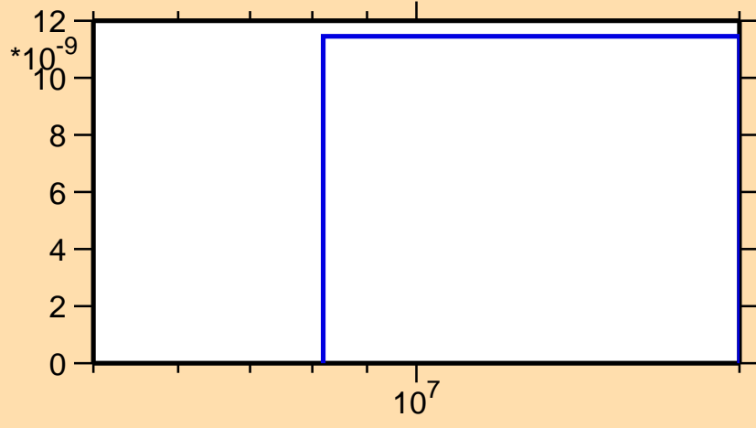
\sigma vs. E for ^{202}\text{Po}(n,p\alpha)
