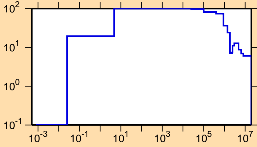
\Delta\sigma/\sigma vs. E for ^{202}\text{Po}(n,\text{nonel.})
