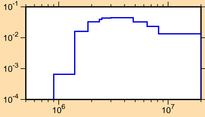
\sigma vs. E for ^{202}\text{Po}(n,n_2)
