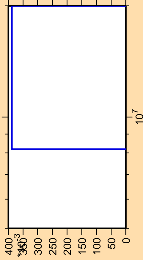
\Delta\sigma/\sigma vs. E for ^{202}\text{Po} (mt 45)
