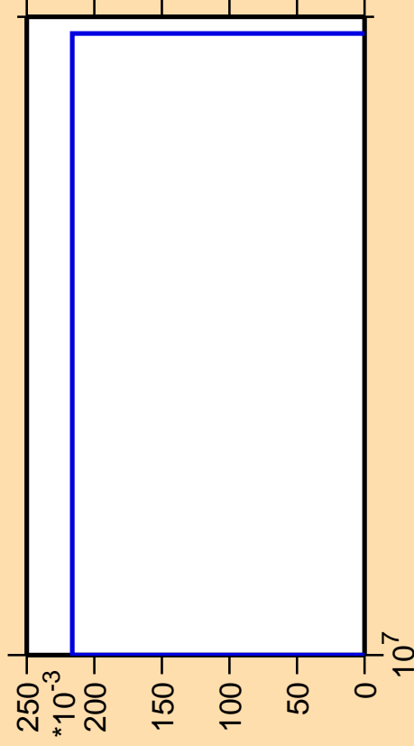
\Delta\sigma/\sigma vs. E for ^{203}\text{Po} (mt 45)
