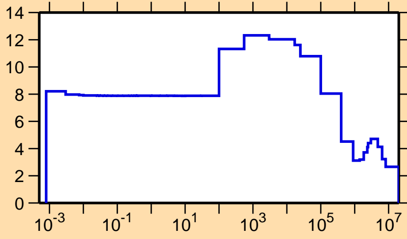
\sigma vs. E for ^{203}\text{Po}(n,\text{el.})
