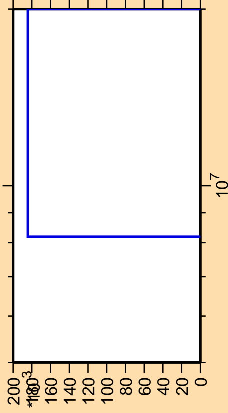
\Delta\sigma/\sigma vs. E for ^{203}\text{Po}(\text{mt } 45)
