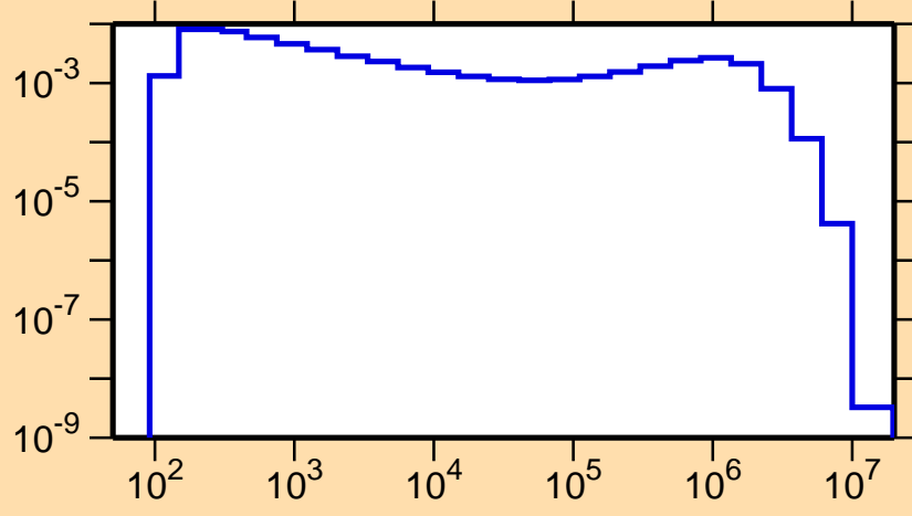
\sigma vs. E for ^{203}\text{Po}(n,n_1)
