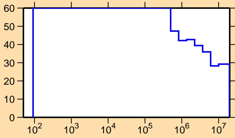
\Delta\sigma/\sigma vs. E for ^{203}\text{Po}(n,n_1)
