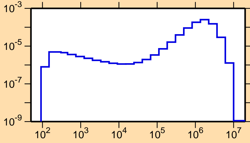
\sigma vs. E for ^{203}\text{Po}(n,n_3)
