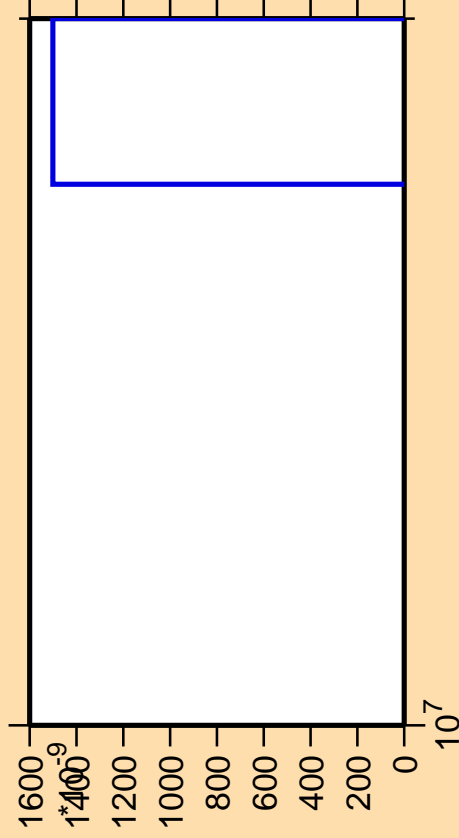
\Delta\sigma/\sigma vs. E for ^{204}\text{Po}(\text{mt 11})
