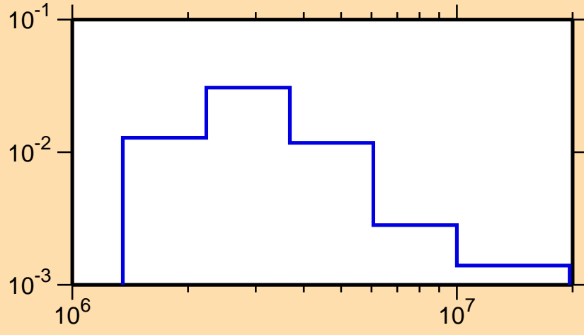
\sigma vs. E for ^{204}\text{Po}(n,n_4)
