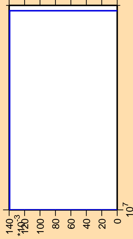
\Delta\sigma/\sigma vs. E for ^{204}\text{Po}(\text{mt } 45)
