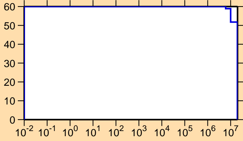
\Delta\sigma/\sigma vs. E for ^{204}\text{Po}(n,p)
