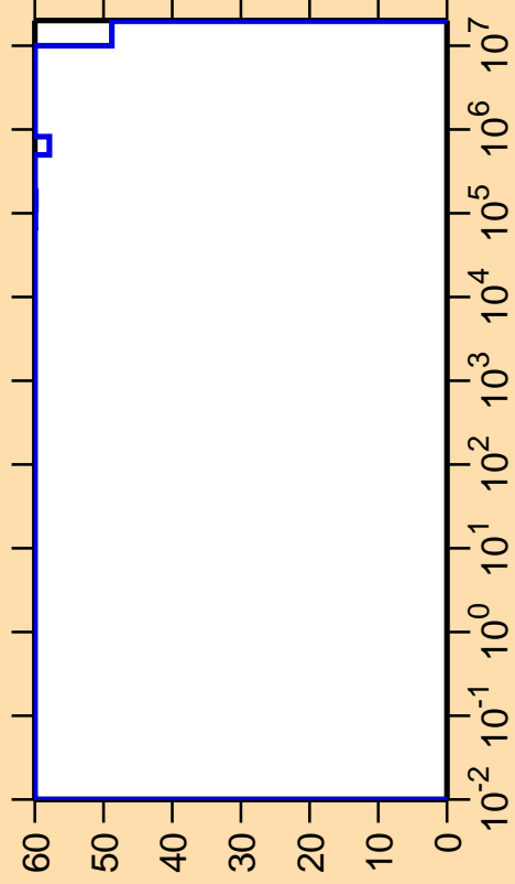
\Delta\sigma/\sigma vs. E for ^{204}\text{Po}(n,\alpha)
