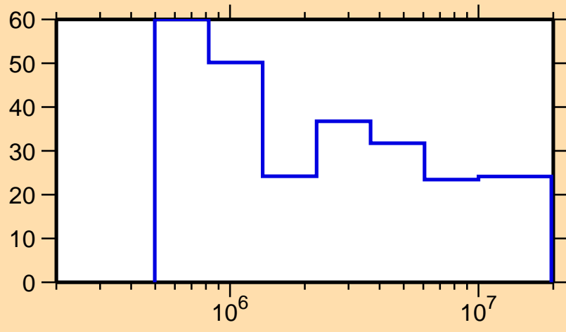
\Delta\sigma/\sigma vs. E for ^{204}\text{Po}(n,n_1)
