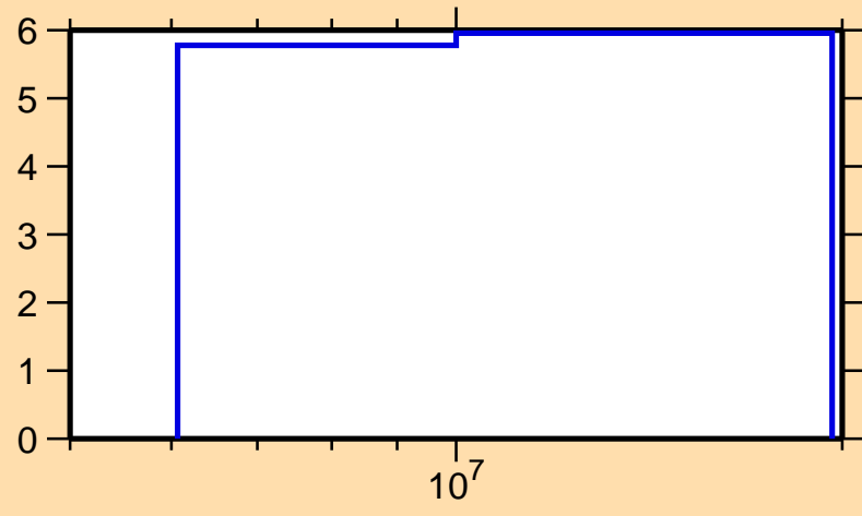
\Delta\sigma/\sigma vs. E for ^{204}\text{Po}(n,\text{nonel.})
