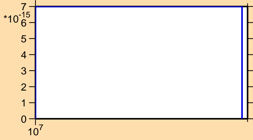
\sigma vs. E for ^{204}\text{Po}(n,\text{pt})
