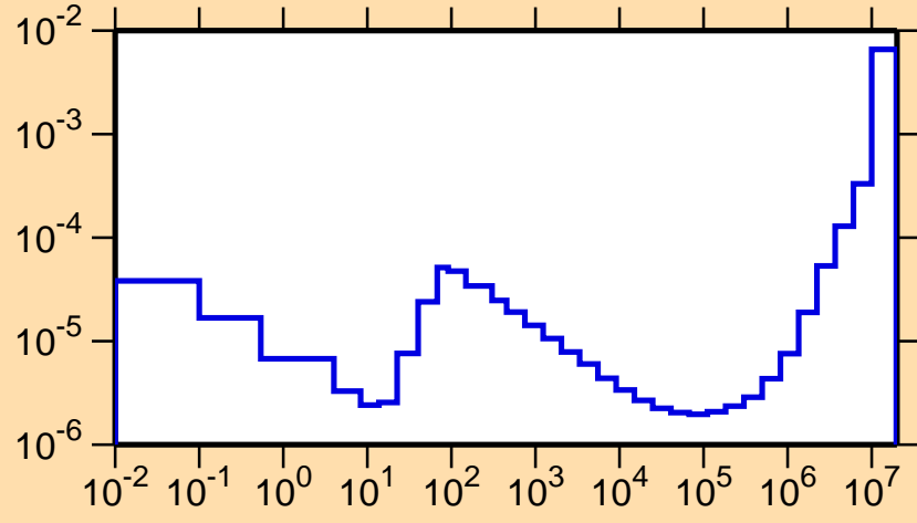
\sigma vs. E for ^{204}\text{Po}(n,\alpha)
