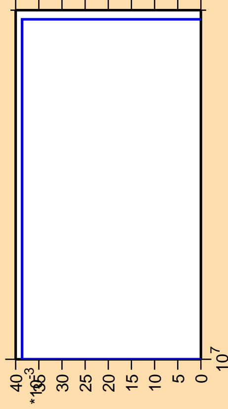
\Delta\sigma/\sigma vs. E for ^{204}\text{Po}(\text{mt117})
