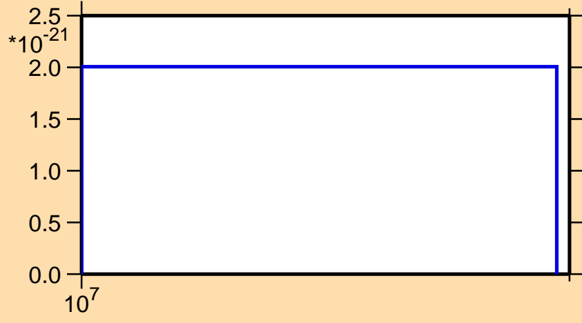
\sigma vs. E for ^{204}\text{Po} (mt 11)
