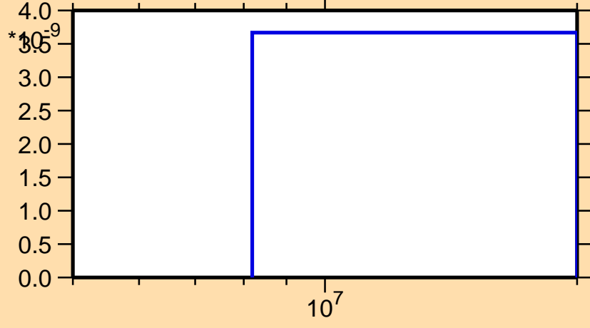
\sigma vs. E for ^{204}\text{Po}(n,p\alpha)
