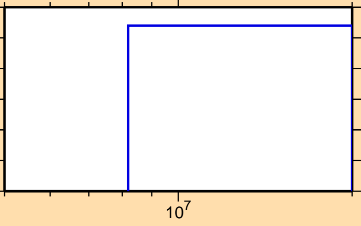
\sigma vs. E for ^{204}\text{Po}(n,2np)
