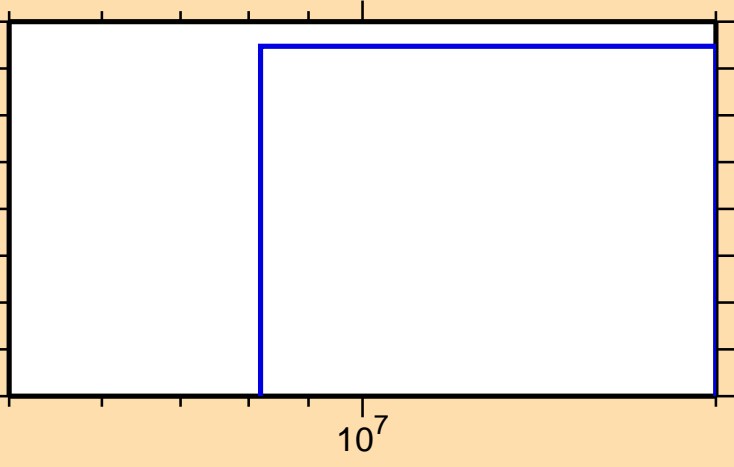
\sigma vs. E for ^{204}\text{Po}(\text{mt117})
