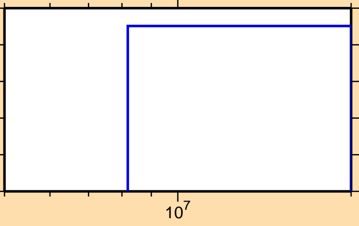
\sigma vs. E for ^{204}\text{Po}(n,\text{He}3)
