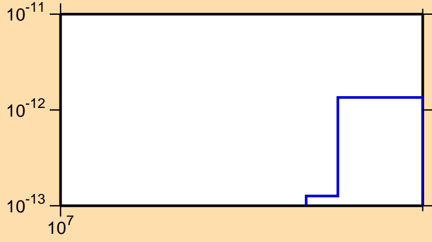
\sigma vs. E for ^{205}\text{Po}(\text{mt117})
