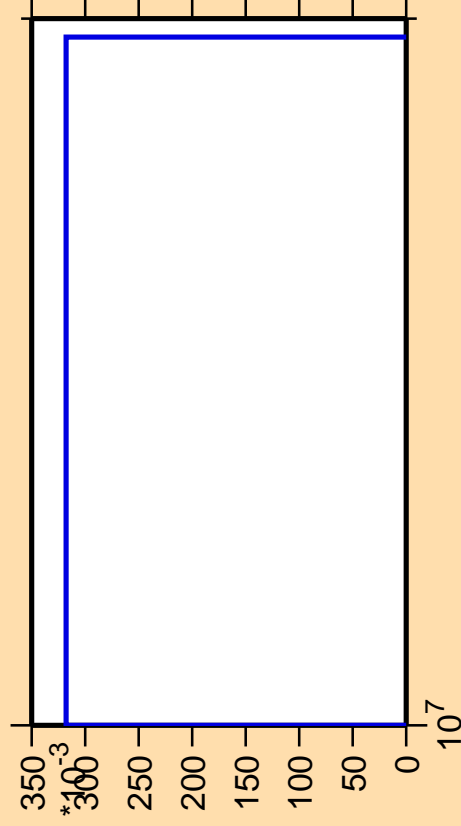
\Delta\sigma/\sigma vs. E for ^{205}\text{Po} (mt 45)
