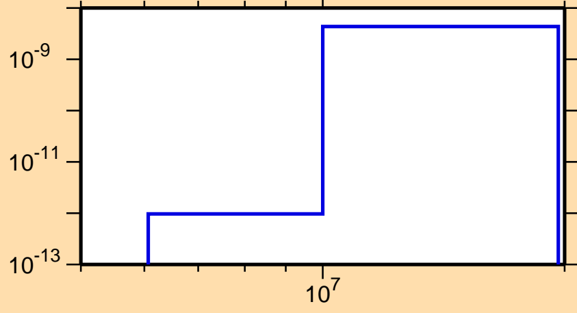
\sigma vs. E for ^{205}\text{Po}(n,p\alpha)
