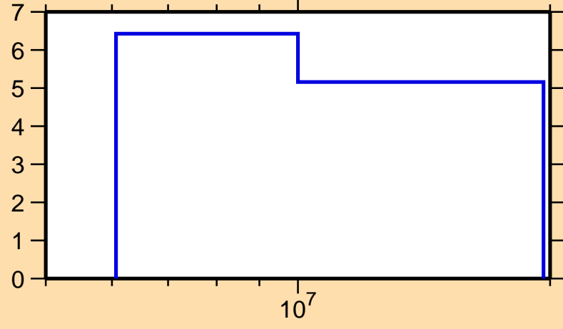
\Delta\sigma/\sigma vs. E for ^{205}\text{Po}(n,\text{nonel.})
