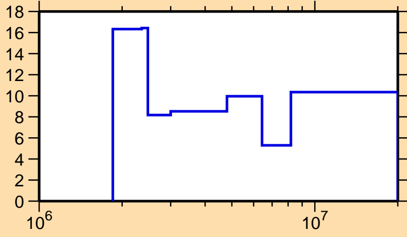
\Delta\sigma/\sigma vs. E for ^{205}\text{Po}(n, el.)
