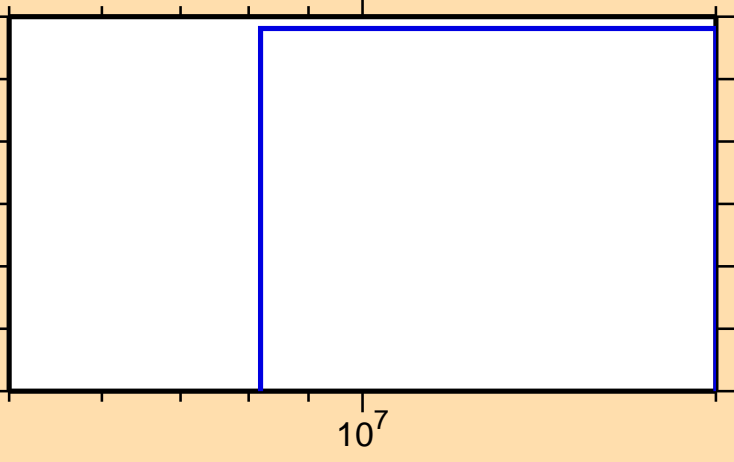
\sigma vs. E for ^{205}\text{Po}(n,\text{nd})
