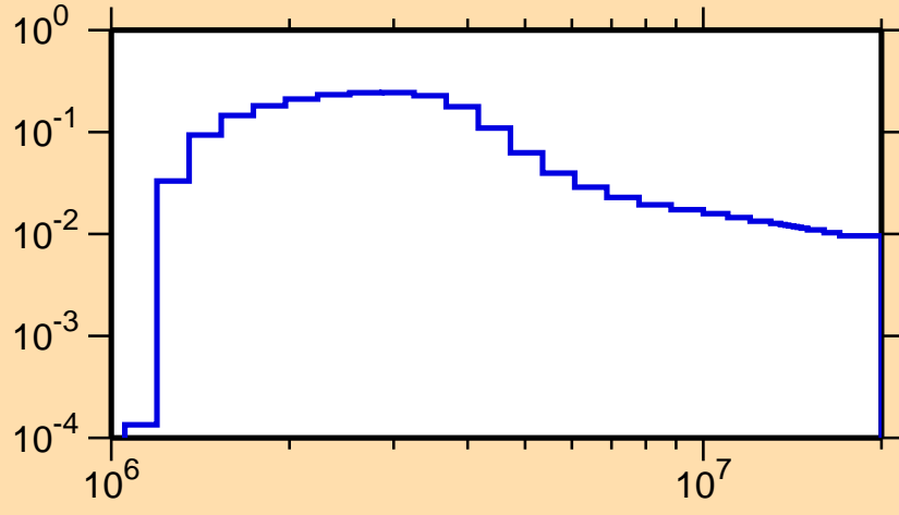
\sigma vs. E for ^{206}\text{Po}(n,n_3)
