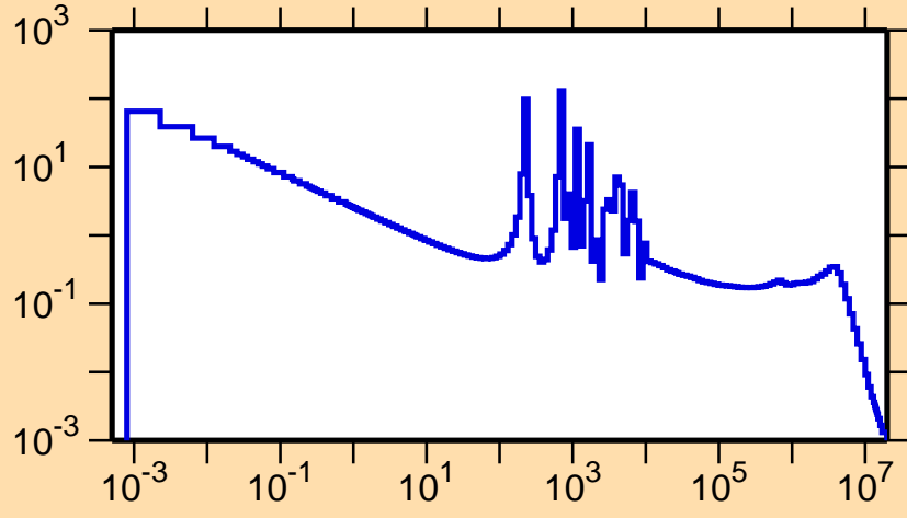
\sigma vs. E for ^{206}\text{Po}(n,\gamma)
