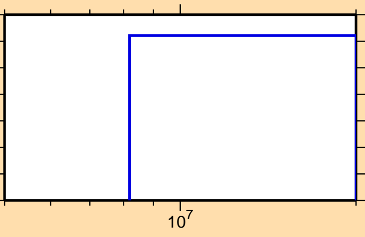
\sigma vs. E for ^{206}\text{Po}(n,\text{pd})
