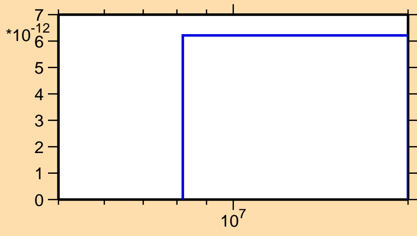
\sigma vs. E for ^{206}\text{Po}(n,\text{pd})
