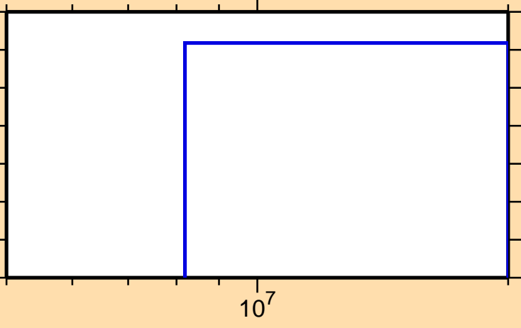
\sigma vs. E for ^{206}\text{Po}(n,3n\alpha)
