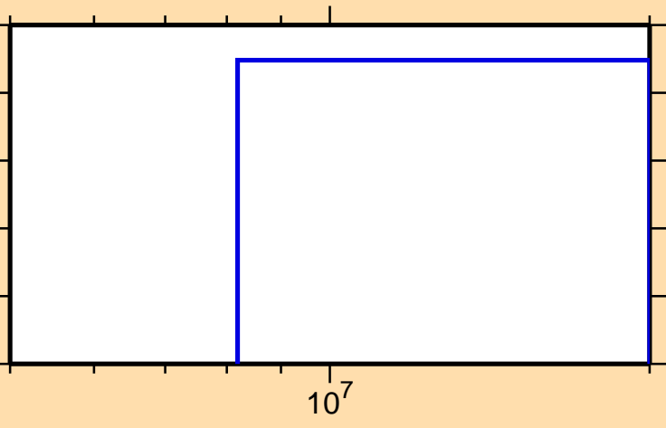
\sigma vs. E for ^{206}\text{Po}(n,2np)
