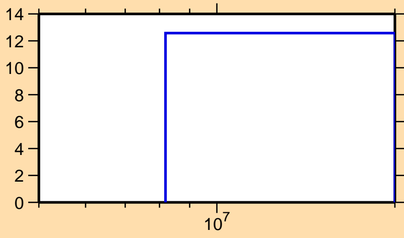
\Delta\sigma/\sigma vs. E for ^{206}\text{Po}(n,2n)
