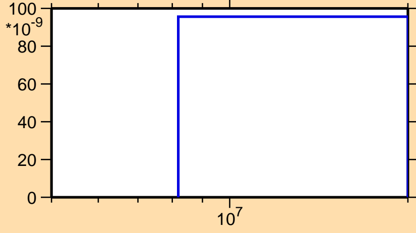
\sigma vs. E for ^{206}\text{Po}(n,2n\alpha)
