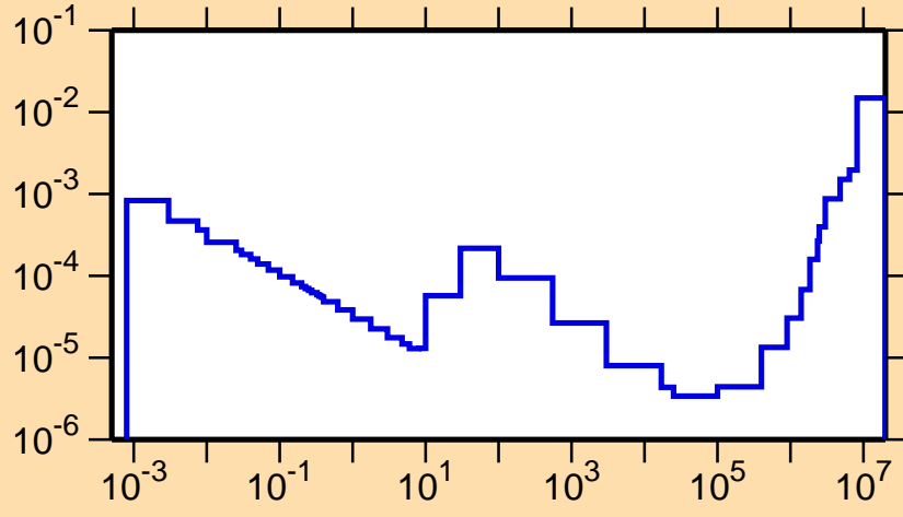
\sigma vs. E for ^{207}\text{Po}(n,p)
