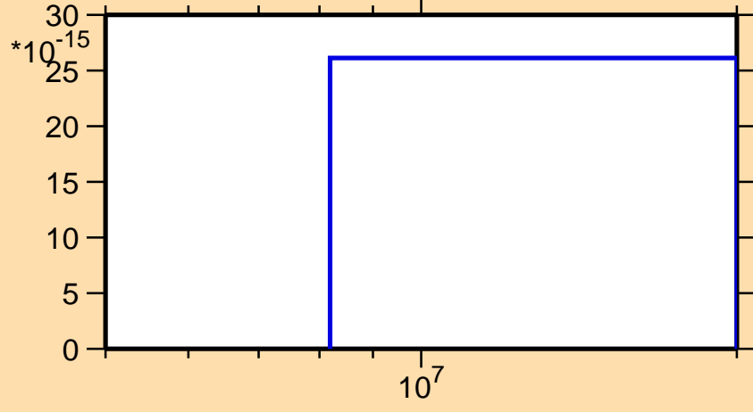
\sigma vs. E for ^{207}\text{Po}(\text{mt } 45)
