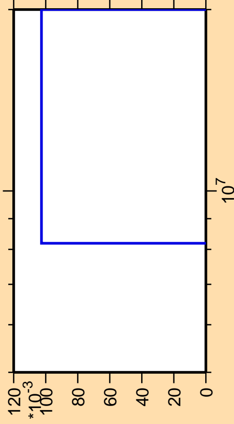
\Delta\sigma/\sigma vs. E for ^{207}\text{Po}(\text{mt } 45)
