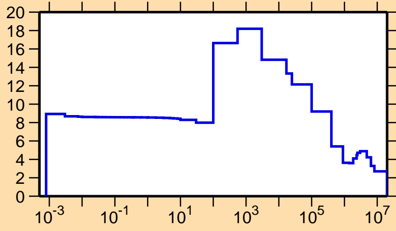
\sigma vs. E for ^{207}\text{Po}(n,\text{el.})
