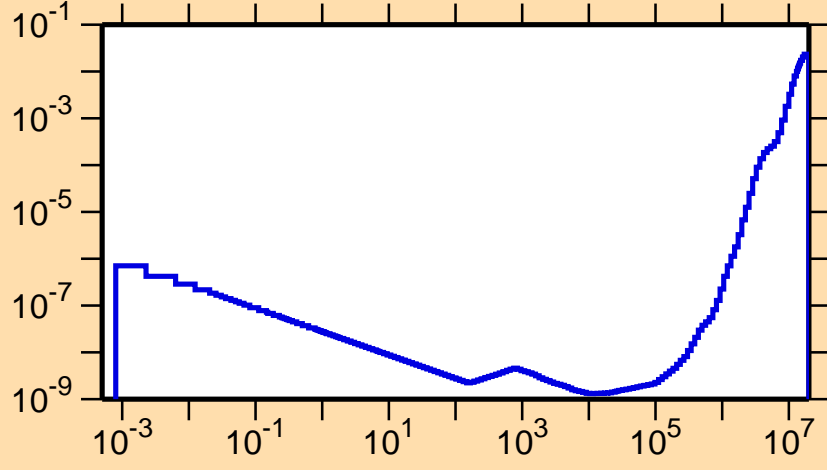
\sigma vs. E for ^{209}\text{Po}(n,p)
