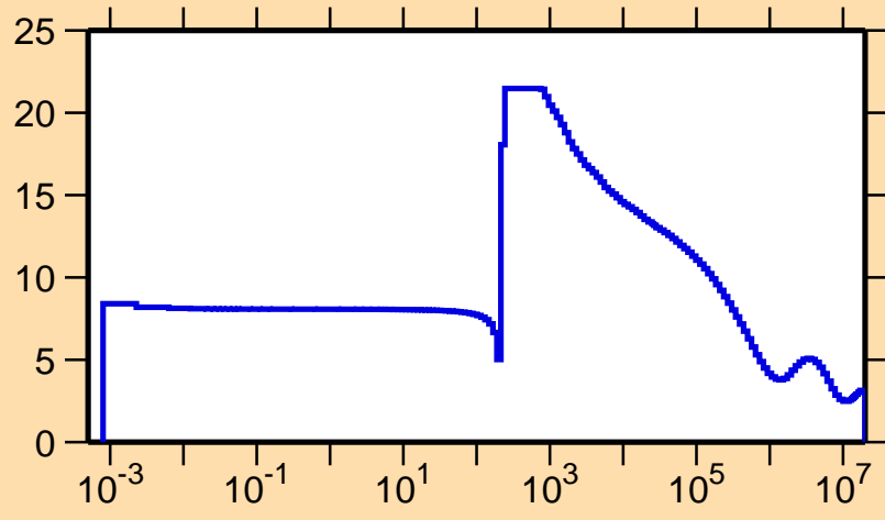
\sigma vs. E for ^{209}\text{Po}(n,\text{el.})
