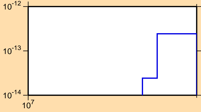
\sigma vs. E for ^{209}\text{Po}(\text{mt 45})
