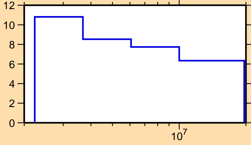
\Delta\sigma/\sigma vs. E for ^{209}\text{Po}(n,n\text{onel.})
