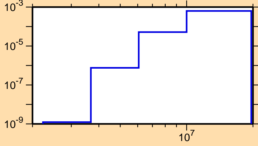
\sigma vs. E for ^{209}\text{Po}(n,n\alpha)
