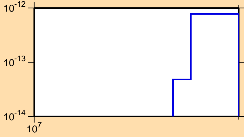
\sigma vs. E for ^{212}\text{Po}(n,\text{pt})
