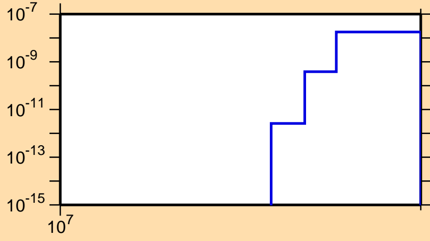
\sigma vs. E for ^{212}\text{Po} (mt 42)
