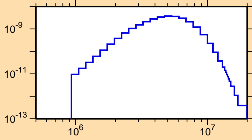
\sigma vs. E for ^{212}\text{Po}(n,n_3)
