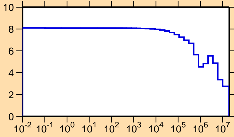
\sigma vs. E for ^{212}\text{Po}(n,\text{el.})
