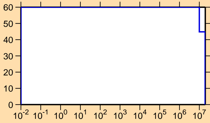
\Delta\sigma/\sigma vs. E for ^{212}\text{Po}(n,\gamma)
