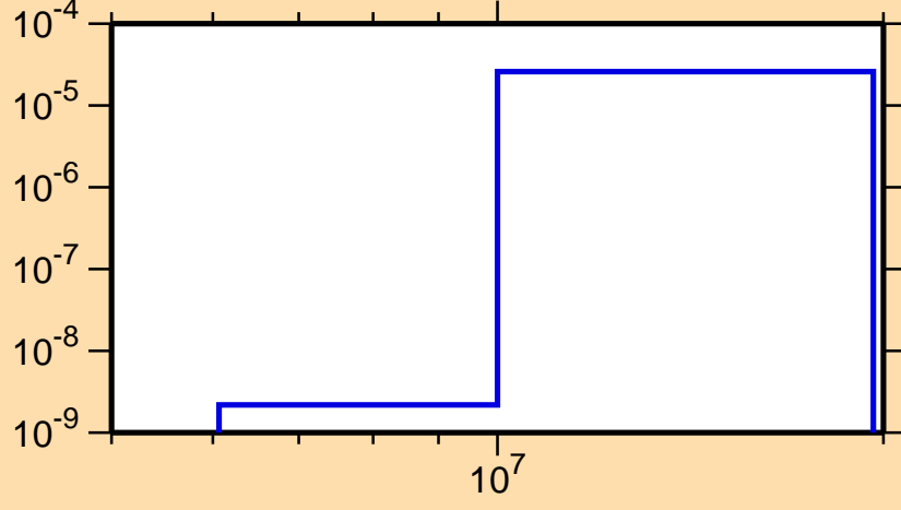
\sigma vs. E for ^{212}\text{Po} (mt 45)
