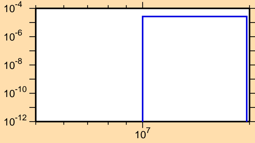
\sigma vs. E for ^{212}\text{Po}(n,nd)
