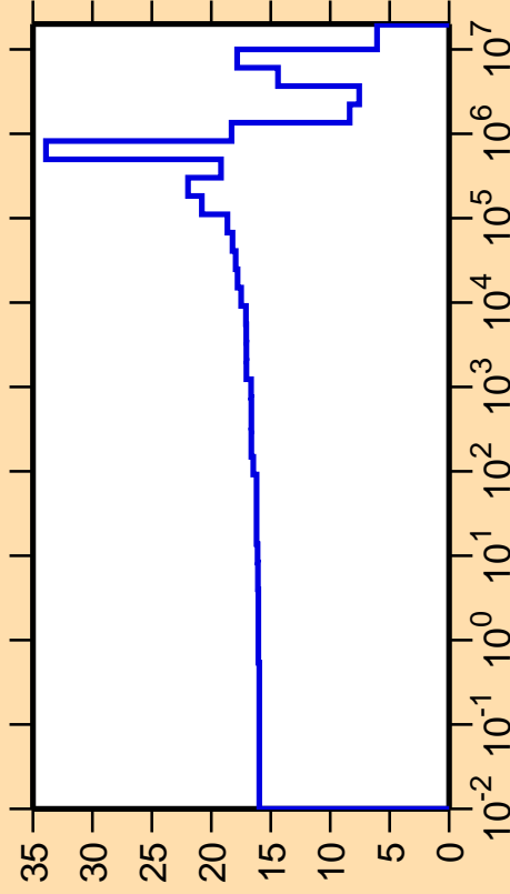
\Delta\sigma/\sigma vs. E for ^{212}\text{Po}(n,\text{el.})
