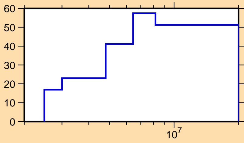
\Delta\sigma/\sigma vs. E for ^{212}\text{Po}(n,n\text{cont.})
