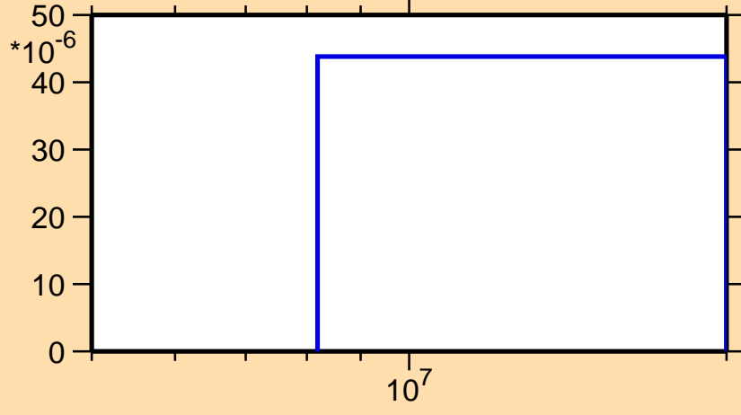
\sigma vs. E for ^{212}\text{Po}(n,nt)
