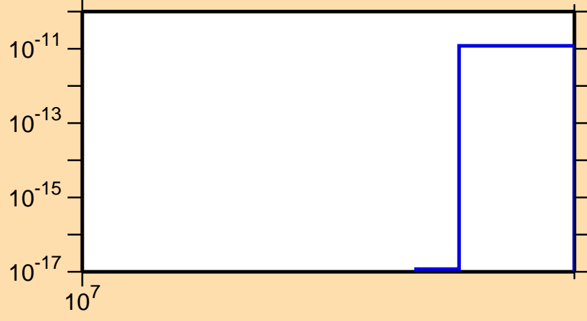
\sigma vs. E for ^{217}\text{Po}(\text{mt 11})
