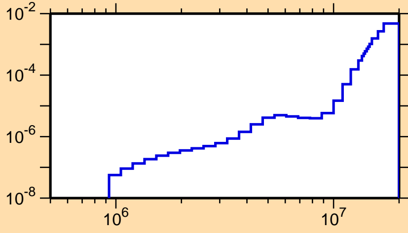
\sigma vs. E for ^{217}\text{Po}(n,n\alpha)
