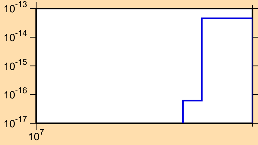
\sigma vs. E for ^{217}\text{Po} (mt 34)
