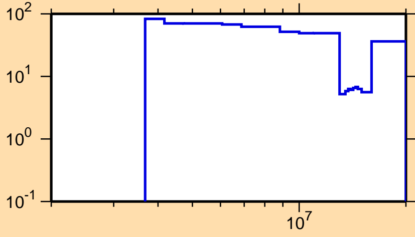
\Delta\sigma/\sigma vs. E for ^{217}\text{Po}(n,2n)
