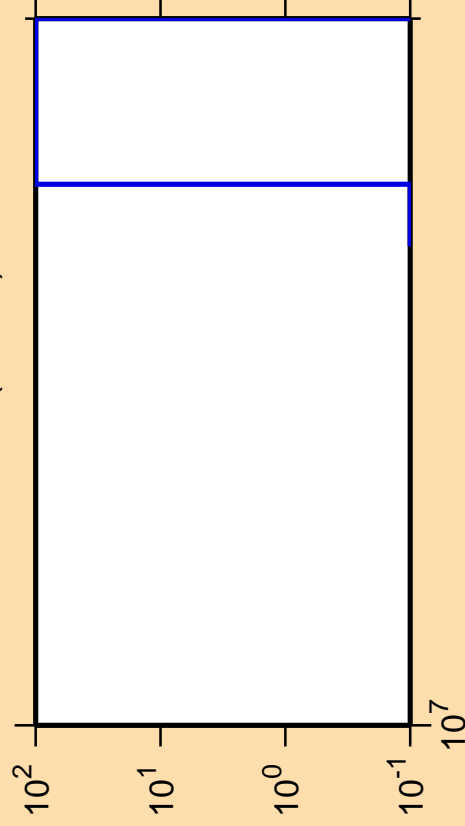
\Delta\sigma/\sigma vs. E for ^{217}\text{Po}(\text{mt 11})
