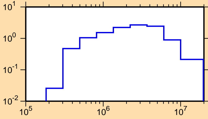
\sigma vs. E for ^{217}\text{Po}(n,\text{inel.})
