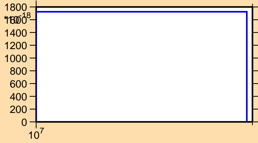
\sigma vs. E for ^{217}\text{Po} (mt 42)
