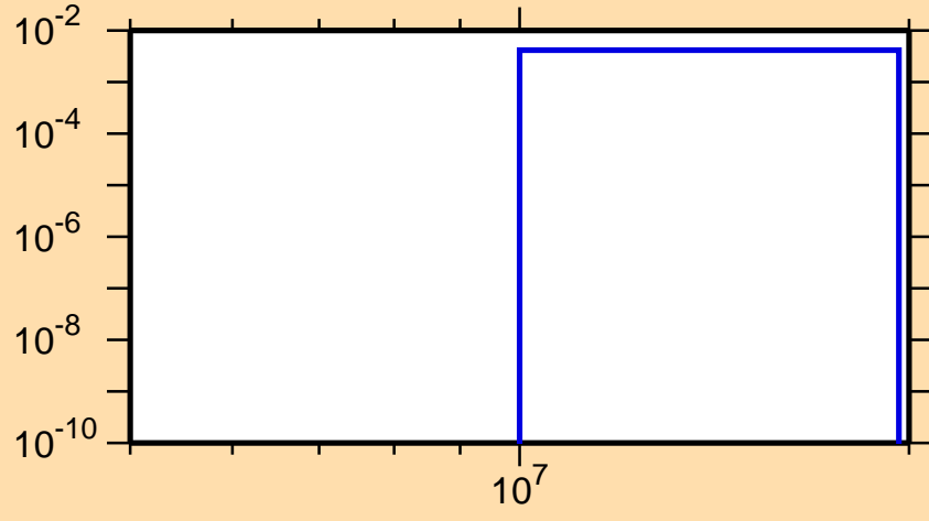
\sigma vs. E for ^{217}\text{Po}(n,3n\alpha)
