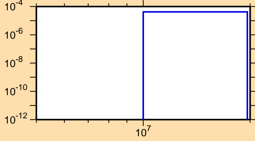
\sigma vs. E for ^{217}\text{Po}(n,np)
