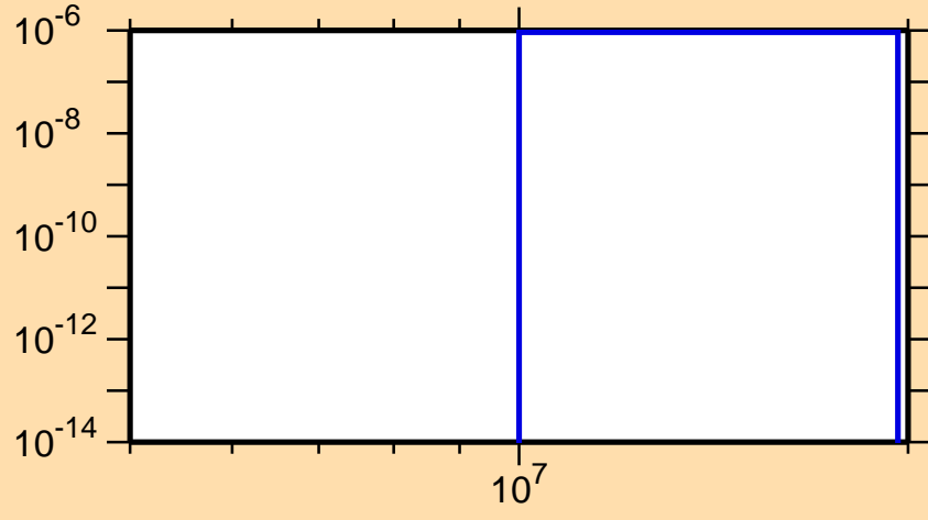
\sigma vs. E for ^{217}\text{Po}(n,nt)
