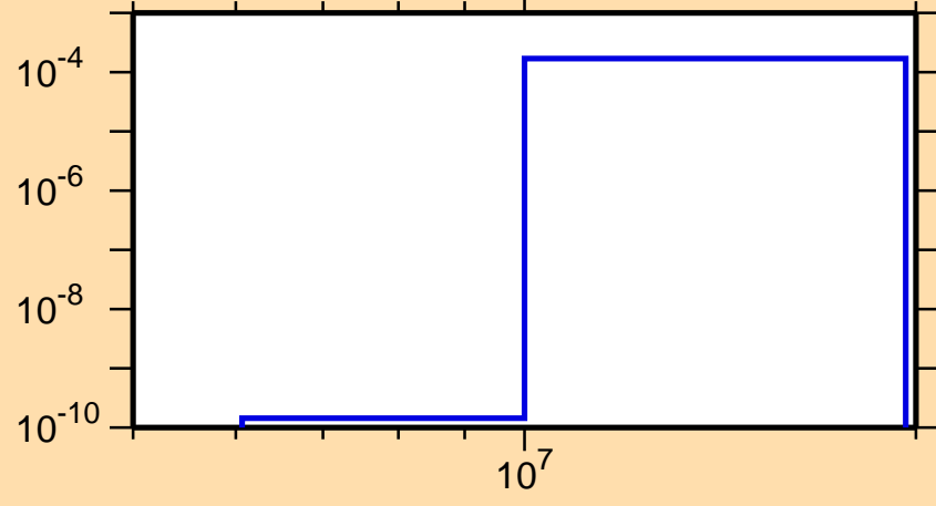
\sigma vs. E for ^{217}\text{Po}(n,t)
