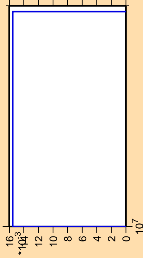
\Delta\sigma/\sigma vs. E for ^{217}\text{Po} (mt 42)
