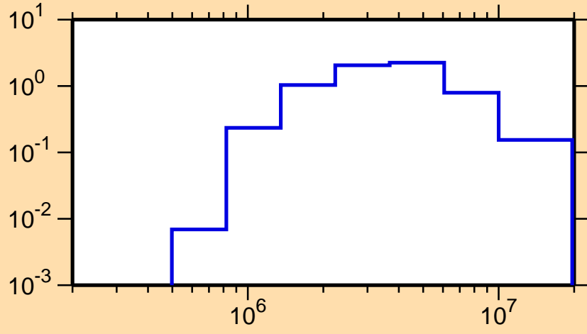
\sigma vs. E for ^{217}\text{Po}(n,n\text{cont.})
