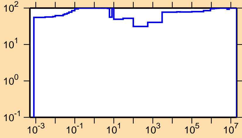
\Delta\sigma/\sigma vs. E for ^{217}\text{Po}(n,\gamma)
