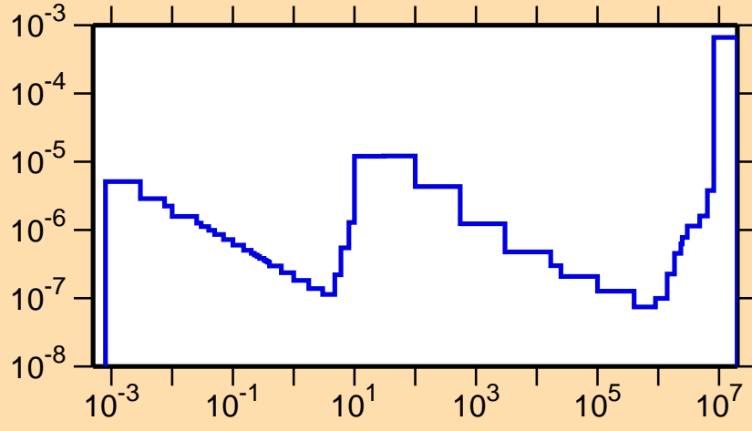
\sigma vs. E for ^{217}\text{Po}(n,\alpha)
