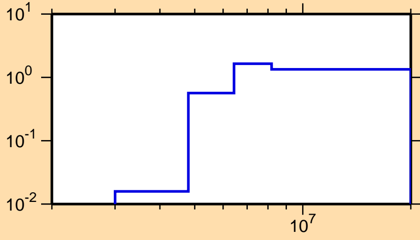
\sigma vs. E for ^{217}\text{Po}(n,2n)
