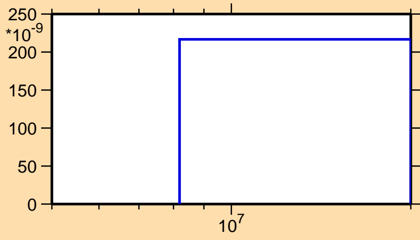
\sigma vs. E for ^{217}\text{Po}(n,\text{nd})
