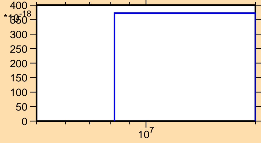
\sigma vs. E for ^{217}\text{Po}(\text{mt } 34)
