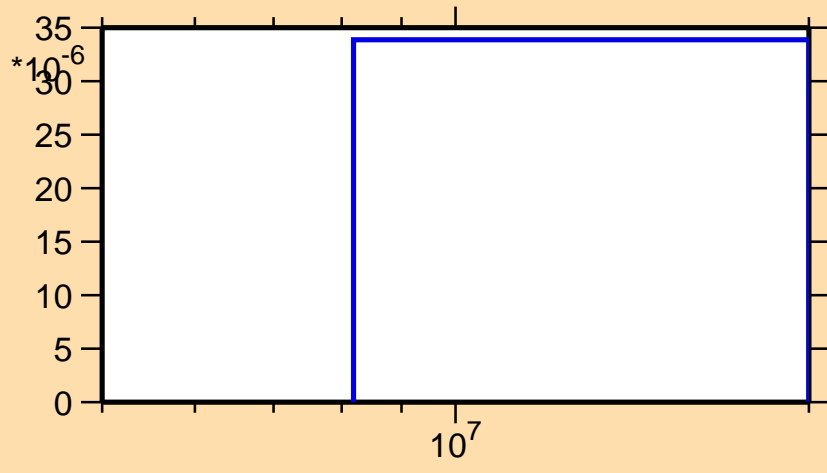
\sigma vs. E for ^{217}\text{Po}(n,np)
