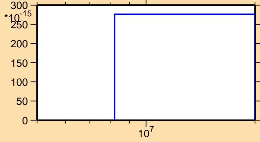
\sigma vs. E for ^{217}\text{Po}(n,\text{He3})
