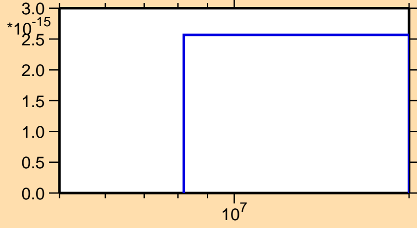
\sigma vs. E for ^{217}\text{Po}(\text{mt } 42)
