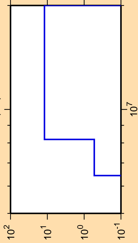
\Delta\sigma/\sigma vs. E for ^{217}\text{Po}(n,t)
