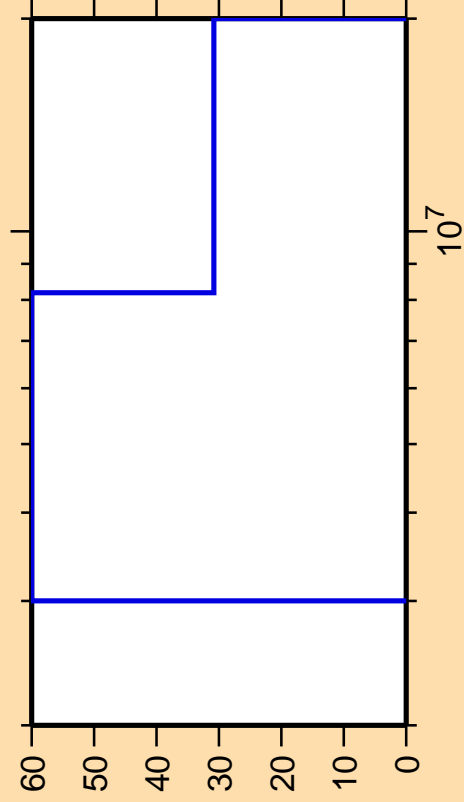
\Delta\sigma/\sigma vs. E for ^{217}\text{Po}(n,2n)
