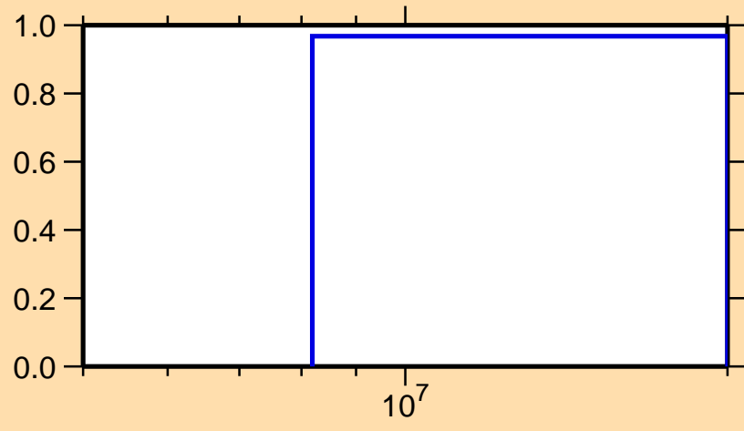
\sigma vs. E for ^{217}\text{Po}(n,3n)
