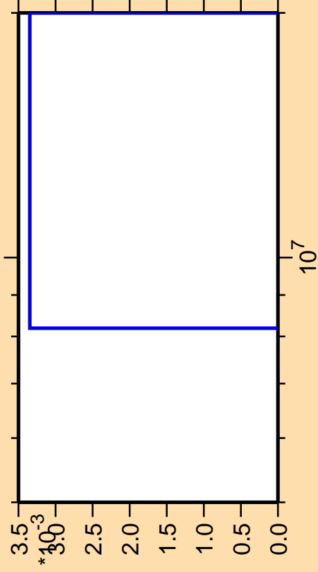
\Delta\sigma/\sigma vs. E for ^{217}\text{Po}(\text{mt } 34)
