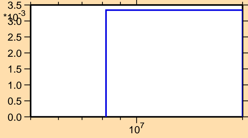
\sigma vs. E for ^{217}\text{Po}(n,3n\alpha)
