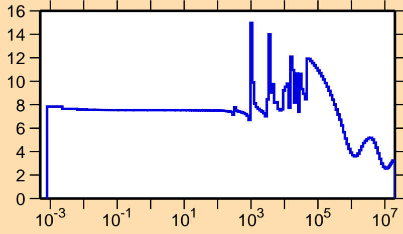
\sigma vs. E for ^{218}\text{Po}(n,\text{el.})
