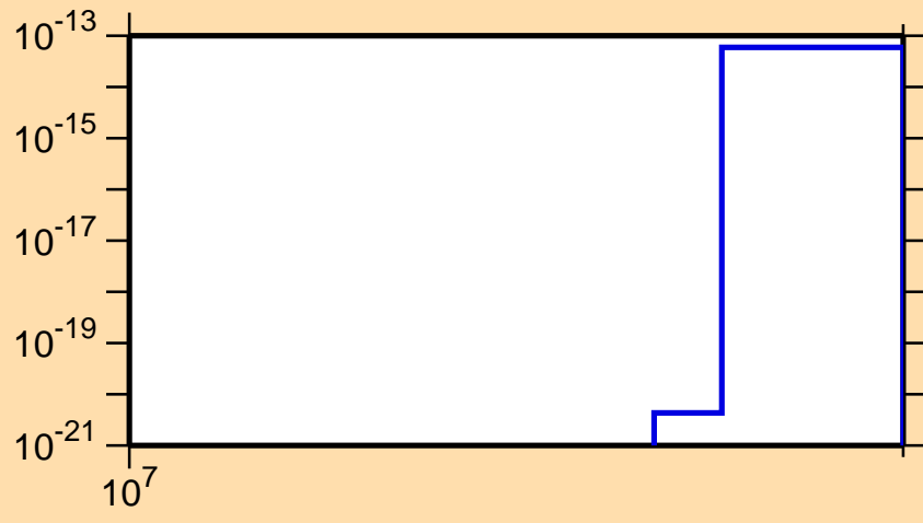
\sigma vs. E for ^{218}\text{Po} (mt 42)
