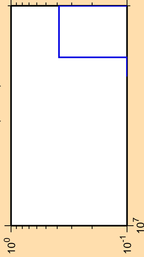
\Delta\sigma/\sigma vs. E for ^{218}\text{Po} (mt 42)
