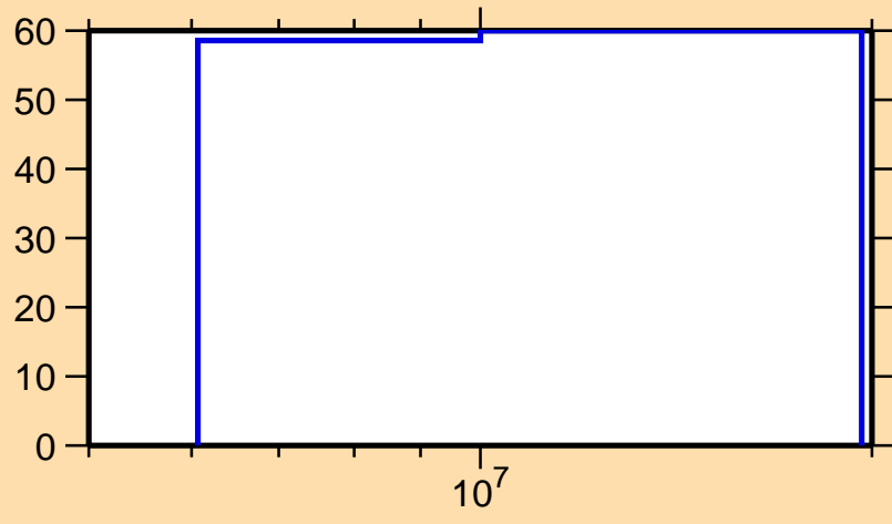
\Delta\sigma/\sigma vs. E for ^{218}\text{Po}(n,el.)
