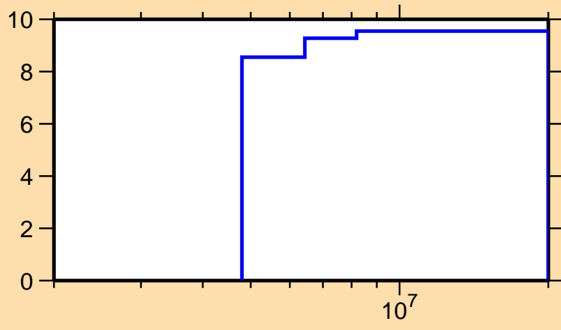
\Delta\sigma/\sigma vs. E for ^{218}\text{Po}(n,\text{nonel.})
