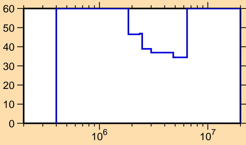
\Delta\sigma/\sigma vs. E for ^{218}\text{Po}(n,\text{el.})
