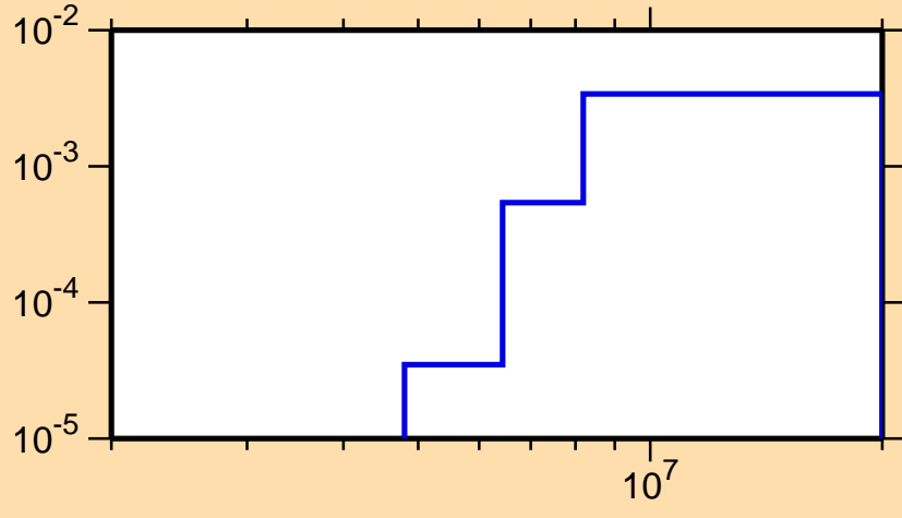
\sigma vs. E for ^{218}\text{Po}(n,2n\alpha)
