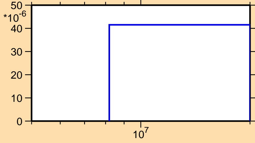
\sigma vs. E for ^{218}\text{Po}(n,t)
