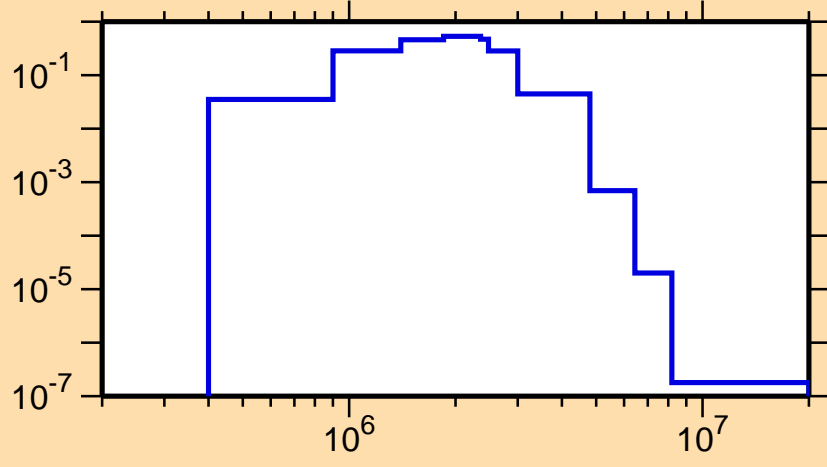
\sigma vs. E for ^{218}\text{Po}(n,n_2)
