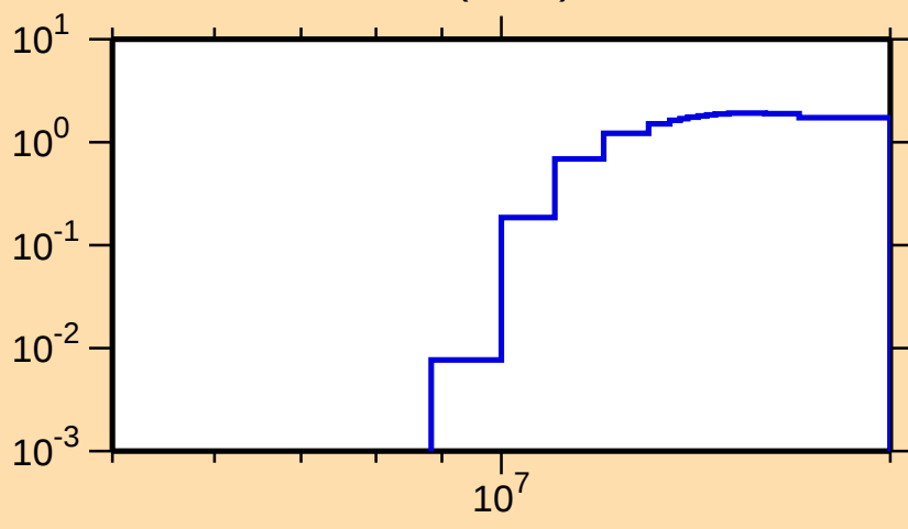
\sigma vs. E for ^{219}\text{Po}(n,3n)
