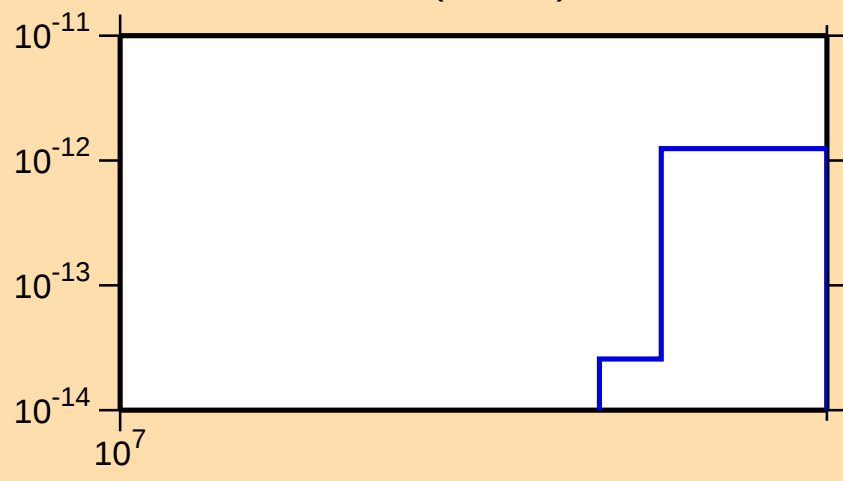
\sigma vs. E for ^{219}\text{Po}(n,\text{He}3)
