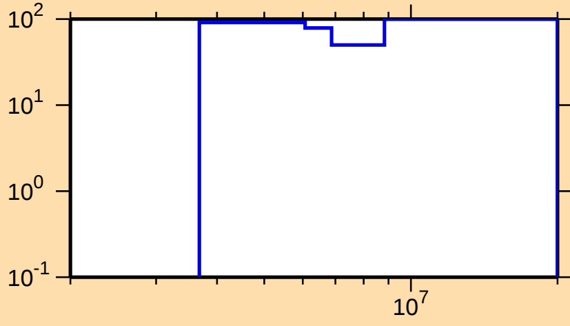
\Delta\sigma/\sigma vs. E for ^{219}\text{Po}(n,2n)
