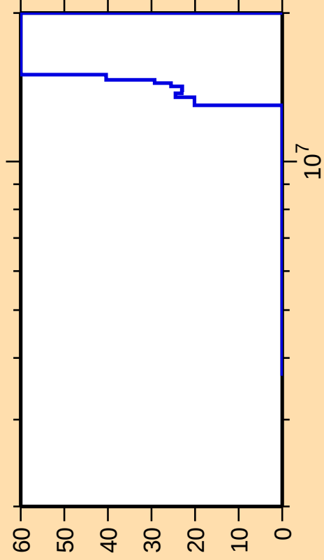
\Delta\sigma/\sigma vs. E for ^{219}\text{Po}(n,f)
