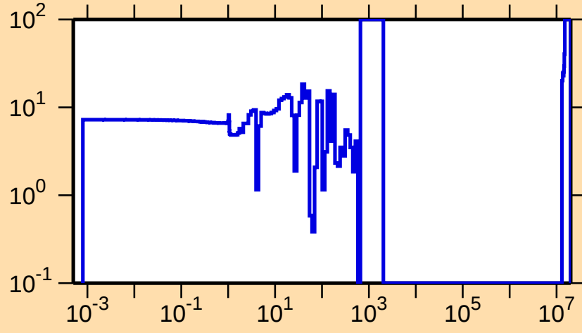
\Delta\sigma/\sigma vs. E for ^{219}\text{Po}(n,f)
