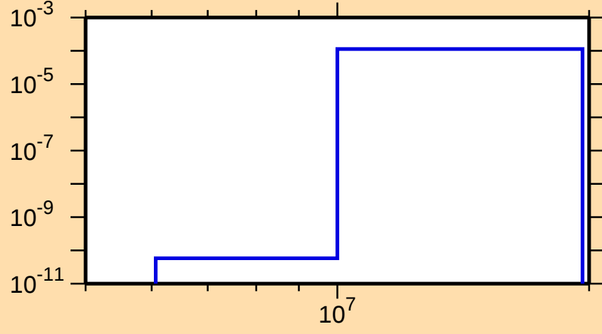
\sigma vs. E for ^{219}\text{Po}(n,t)
