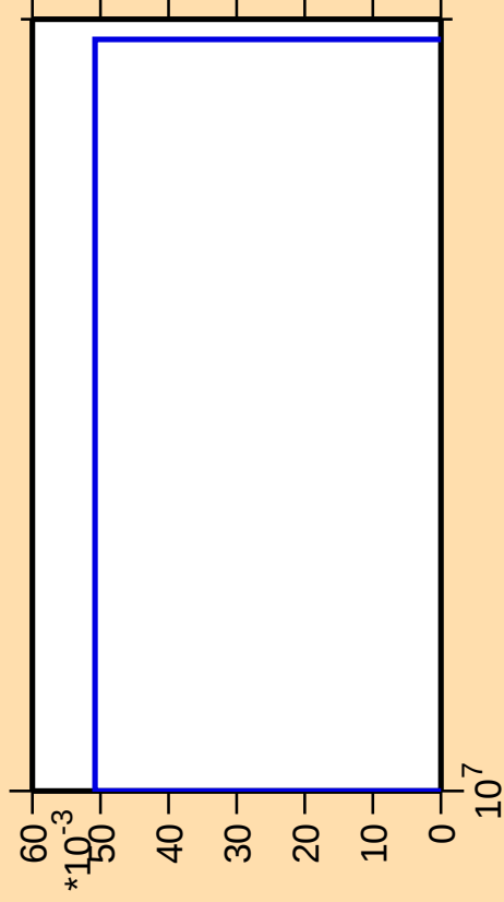
\Delta\sigma/\sigma vs. E for ^{219}\text{Po}(\text{mt 11})
