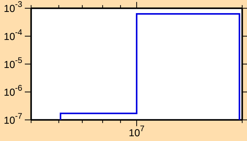
\sigma vs. E for ^{219}\text{Po}(n,p)
