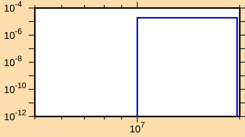
\sigma vs. E for ^{219}\text{Po}(n,np)
