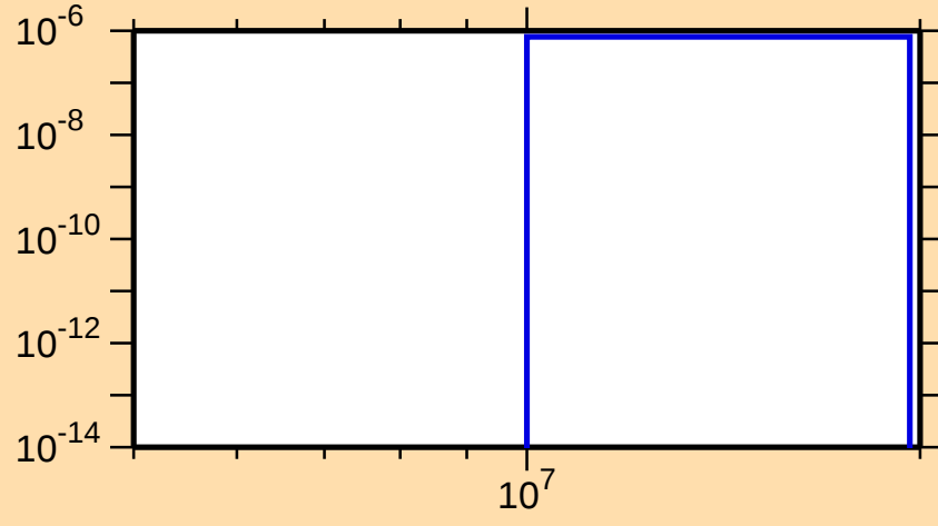
\sigma vs. E for ^{219}\text{Po}(n,nt)
