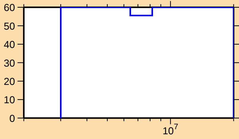
\Delta\sigma/\sigma vs. E for ^{219}\text{Po}(n,2n)
