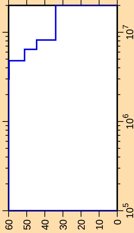
\Delta\sigma/\sigma vs. E for ^{219}\text{Po}(n,n_1)
