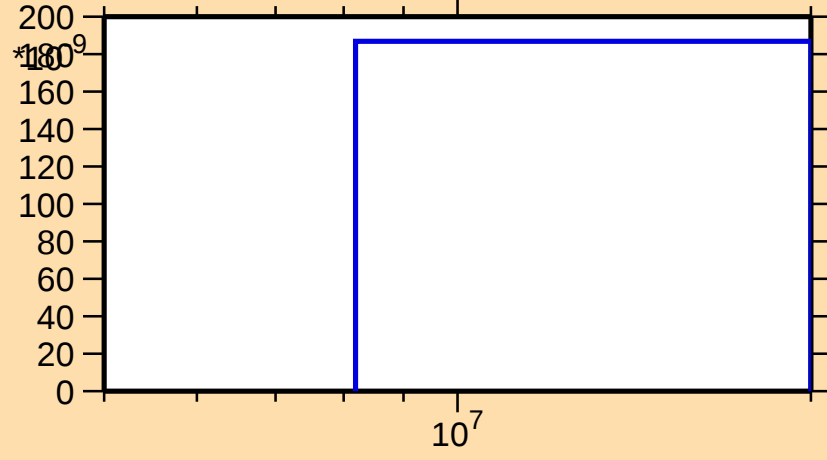
\sigma vs. E for ^{219}\text{Po}(n,\text{nd})
