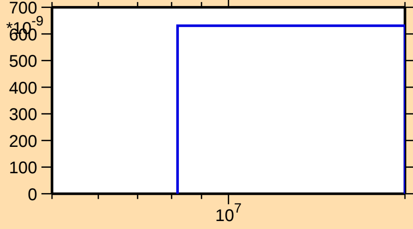
\sigma vs. E for ^{219}\text{Po}(n,nt)
