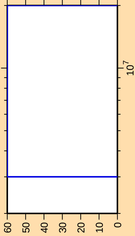
\Delta\sigma/\sigma vs. E for ^{219}\text{Po}(n,n\text{cont.})
