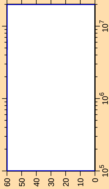
\Delta\sigma/\sigma vs. E for ^{219}\text{Po}(n,\gamma)
