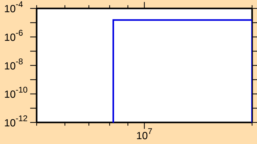
\sigma vs. E for ^{219}\text{Po}(n,np)
