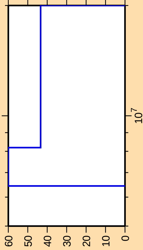
\Delta\sigma/\sigma vs. E for ^{219}\text{Po}(n,p)
