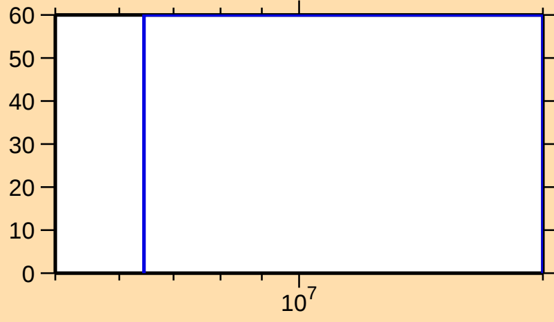
\Delta\sigma/\sigma vs. E for ^{219}\text{Po}(n,\text{ncont.})
