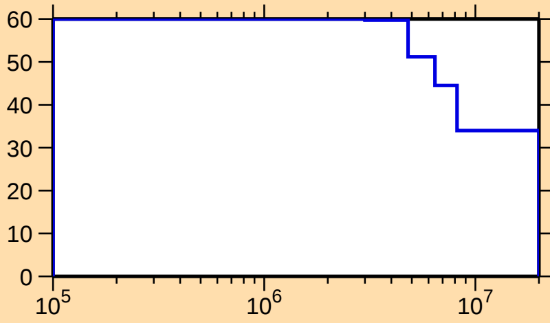
\Delta\sigma/\sigma vs. E for ^{219}\text{Po}(n,n_1)
