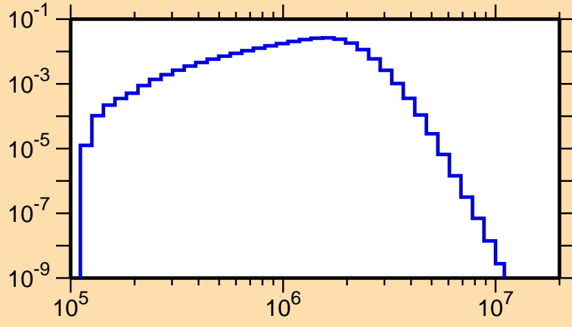
\sigma vs. E for ^{221}\text{Po}(n,n_1)
