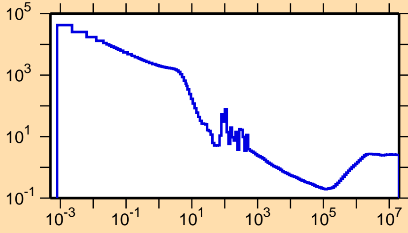
\sigma vs. E for ^{221}\text{Po}(n,\text{nonel.})
