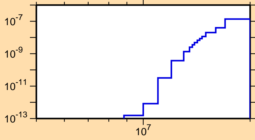
\sigma vs. E for ^{221}\text{Po}(n,3n\alpha)
