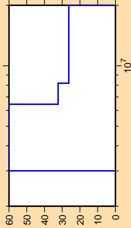
\Delta\sigma/\sigma vs. E for ^{221}\text{Po}(n,2n)
