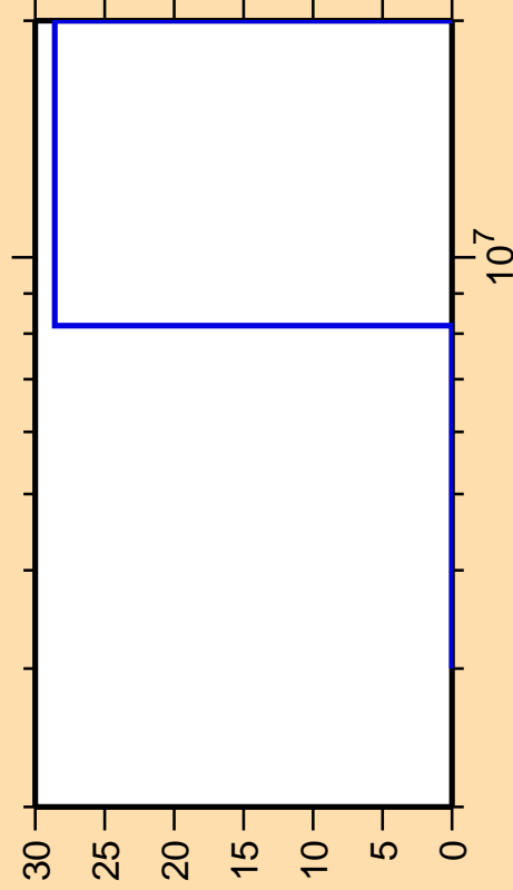
\Delta\sigma/\sigma vs. E for ^{221}\text{Po}(n,f)
