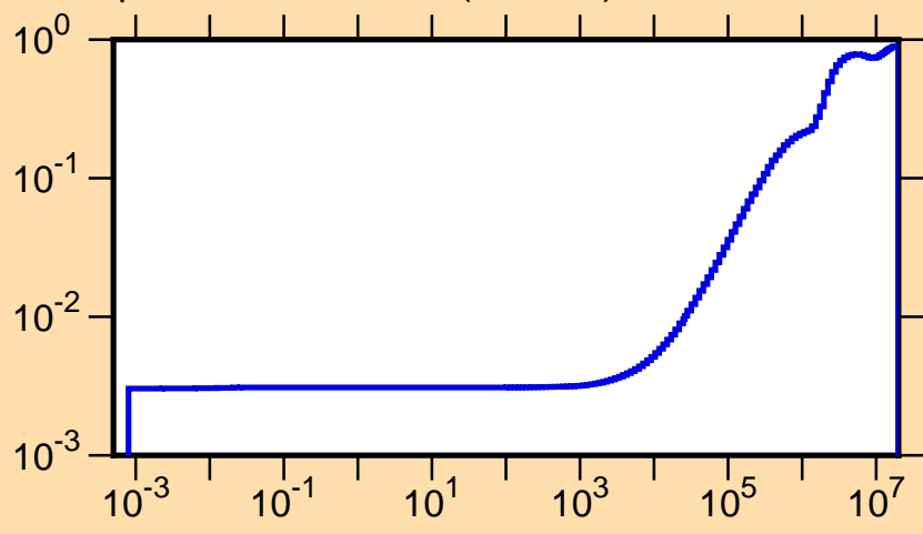
\mu vs. E for ^{222}\text{Po}(\text{mt251})
