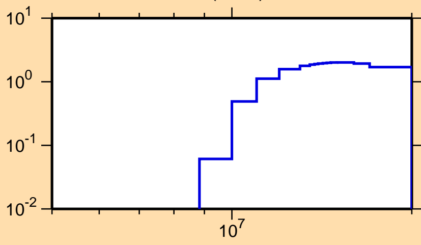
\sigma vs. E for ^{222}\text{Po}(n,3n)
