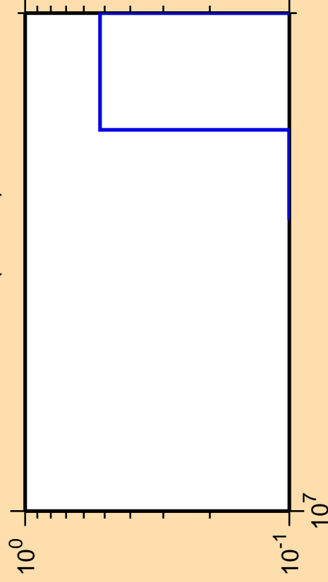
\Delta\sigma/\sigma vs. E for ^{222}\text{Po}(\text{mt } 11)
