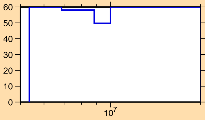
\Delta\sigma/\sigma vs. E for ^{222}\text{Po}(n,2n)
