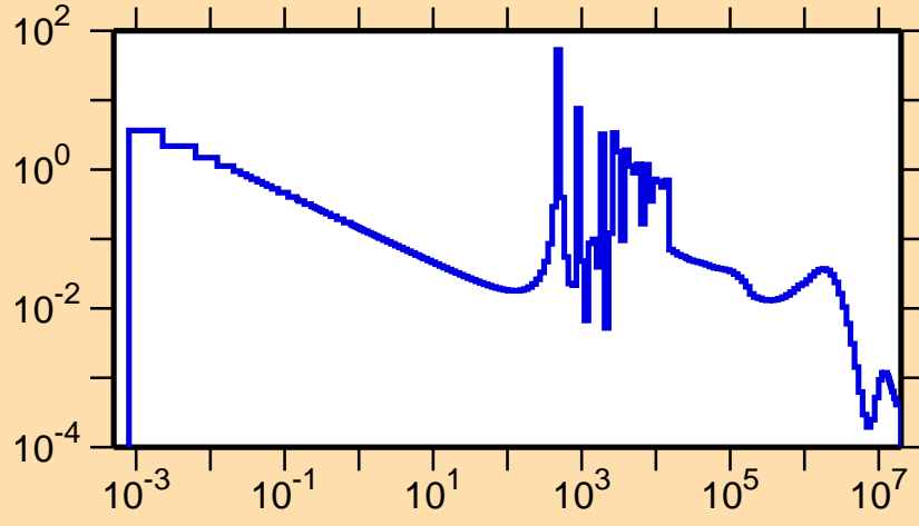
\sigma vs. E for ^{222}\text{Po}(n,\gamma)
