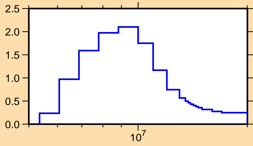
\sigma vs. E for ^{222}\text{Po}(n,2n)
