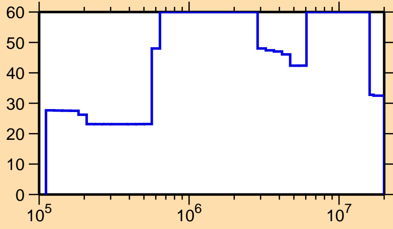
\Delta\sigma/\sigma vs. E for ^{222}\text{Po}(n,\text{el.})
