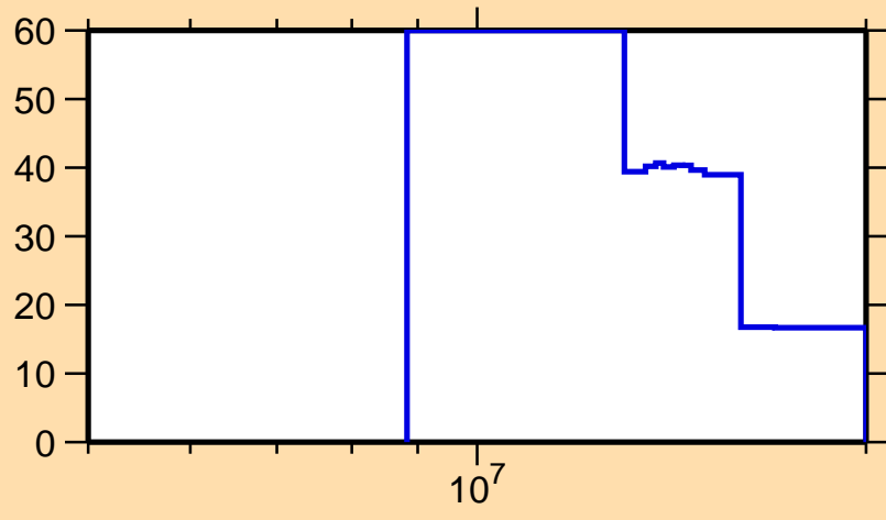
\Delta\sigma/\sigma vs. E for ^{222}\text{Po}(n,\text{tot.})
