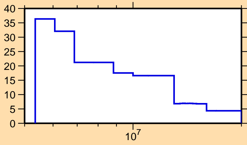
\Delta\sigma/\sigma vs. E for ^{222}\text{Po}(n,\text{nonel.})
