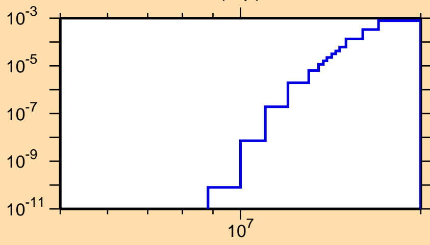
\sigma vs. E for ^{222}\text{Po}(n,p)
