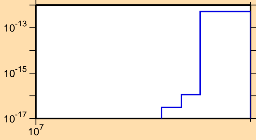
\sigma vs. E for ^{222}\text{Po}(\text{mt } 11)
