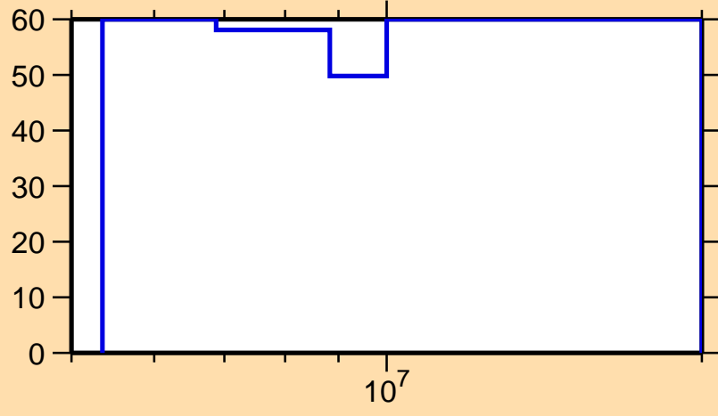
\Delta\sigma/\sigma vs. E for ^{222}\text{Po}(n,2n)
