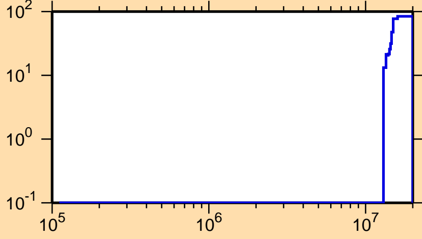
\Delta\sigma/\sigma vs. E for ^{222}\text{Po}(n,f)
