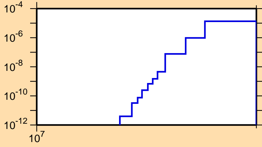
\sigma vs. E for ^{222}\text{Po}(n,nt)
