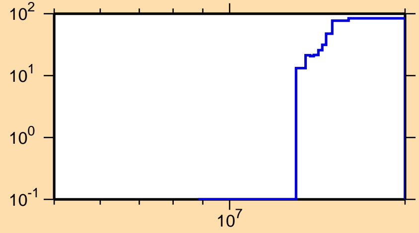
\Delta\sigma/\sigma vs. E for ^{222}\text{Po}(n,f)
