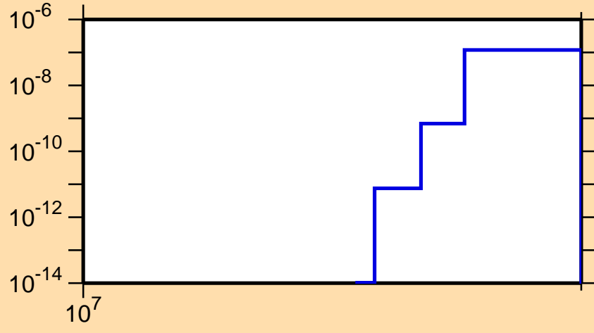
\sigma vs. E for ^{222}\text{Po}(n,\text{nd})
