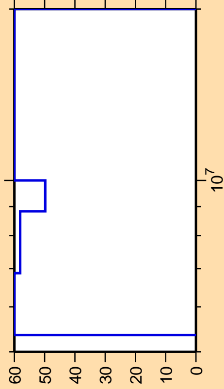
\Delta\sigma/\sigma vs. E for ^{222}\text{Po}(n,2n)
