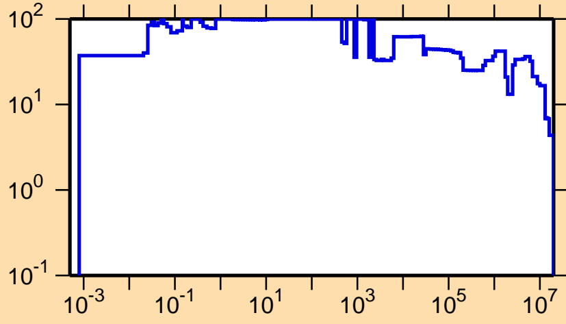
\Delta\sigma/\sigma vs. E for ^{222}\text{Po}(n,\text{nonel.})
