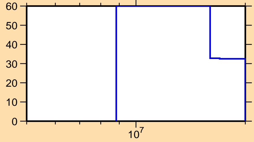
\Delta\sigma/\sigma vs. E for ^{222}\text{Po}(n,el.)
