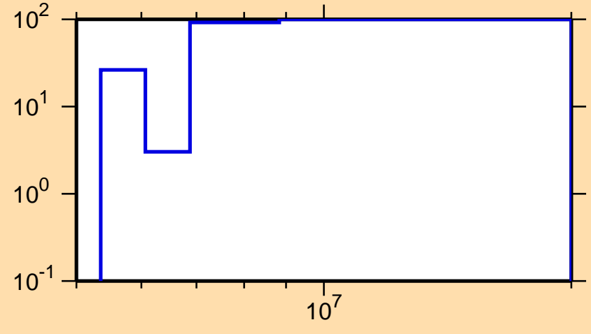
\Delta\sigma/\sigma vs. E for ^{222}\text{Po}(n,\text{inel.})
