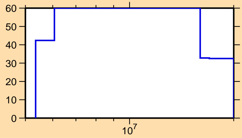
\Delta\sigma/\sigma vs. E for ^{222}\text{Po}(n,\text{el.})
