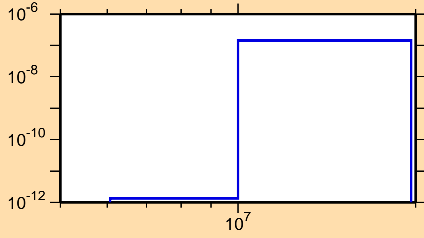
\sigma vs. E for ^{222}\text{Po}(n,2n\alpha)
