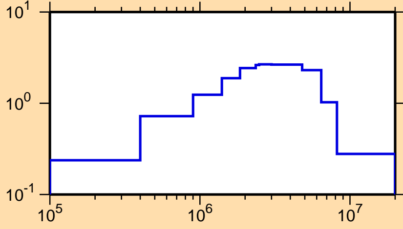
\sigma vs. E for ^{222}\text{Po}(n,\text{inel.})
