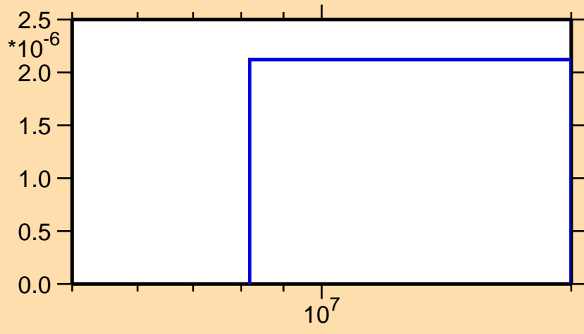
\sigma vs. E for ^{222}\text{Po}(n,np)
