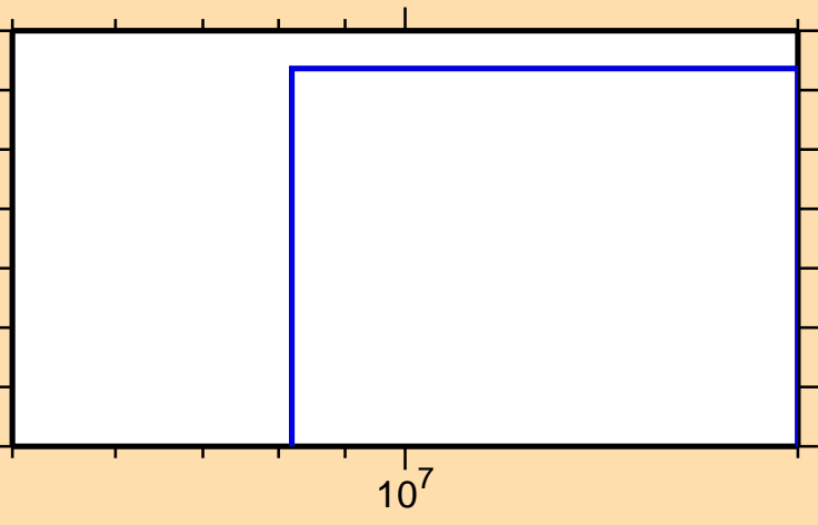
\sigma vs. E for ^{222}\text{Po}(n,t)
