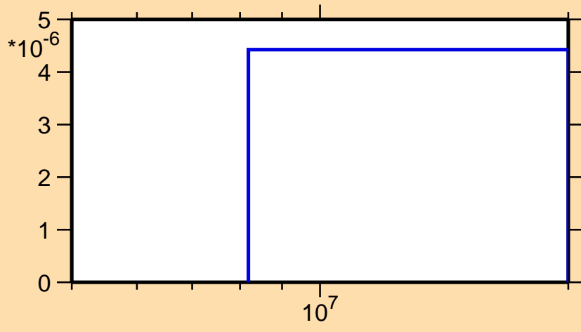
\sigma vs. E for ^{222}\text{Po}(n,d)
