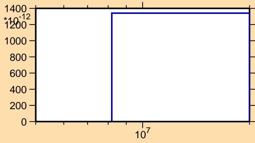
\sigma vs. E for ^{222}\text{Po}(n,3n\alpha)
