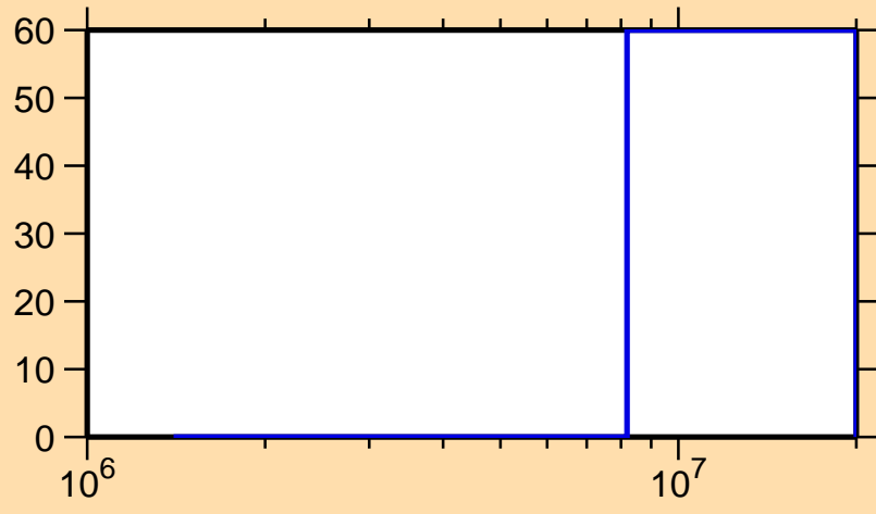
\Delta\sigma/\sigma vs. E for ^{222}\text{Po}(n,f)
