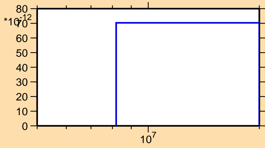
\sigma vs. E for ^{222}\text{Po}(n,2np)
