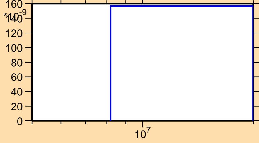
\sigma vs. E for ^{222}\text{Po}(n,nt)
