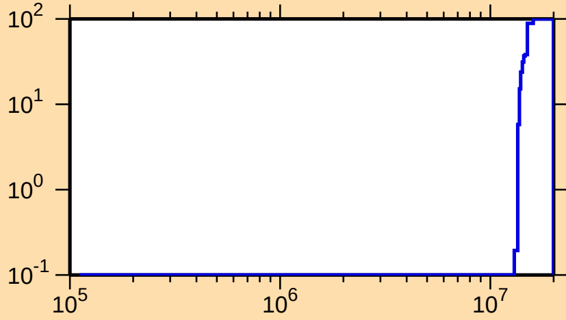
\Delta\sigma/\sigma vs. E for ^{224}\text{Po}(n,\text{f})
