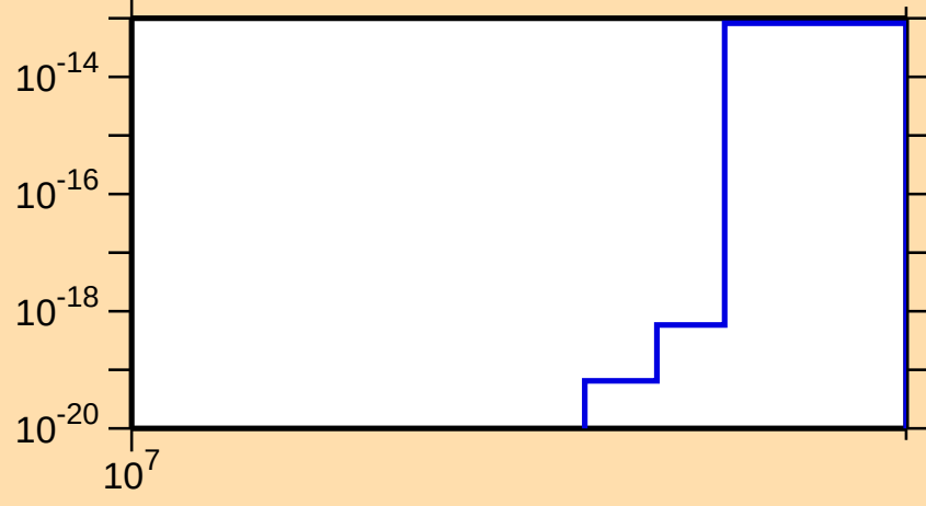
\sigma vs. E for ^{224}\text{Po}(\text{mt } 11)
