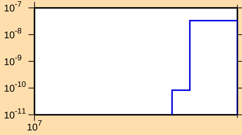
\sigma vs. E for ^{224}\text{Po}(n,\text{nd})
