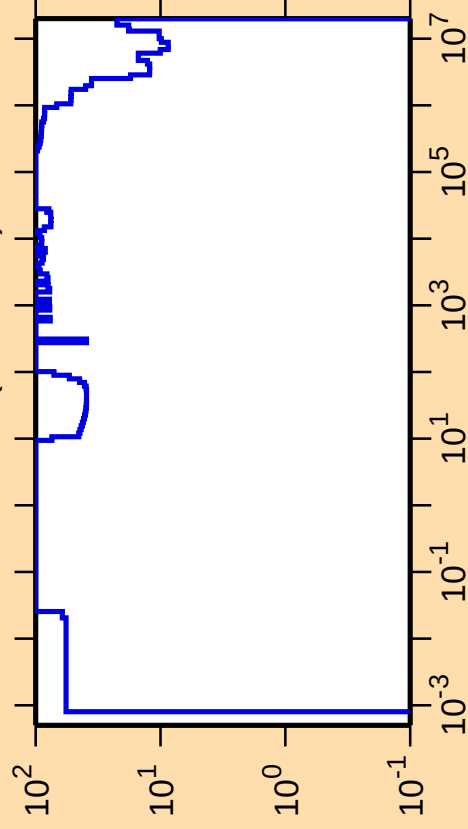
\Delta\sigma/\sigma vs. E for ^{224}\text{Po}(n,\text{nonel.})
