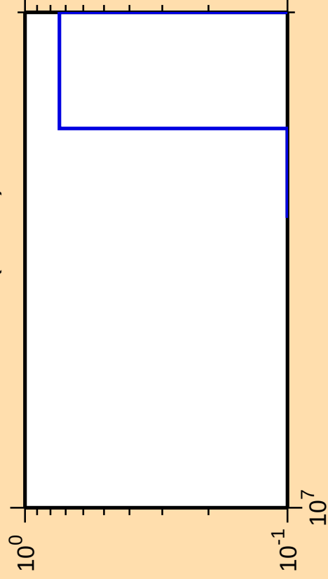
\Delta\sigma/\sigma vs. E for ^{224}\text{Po}(\text{mt } 11)
