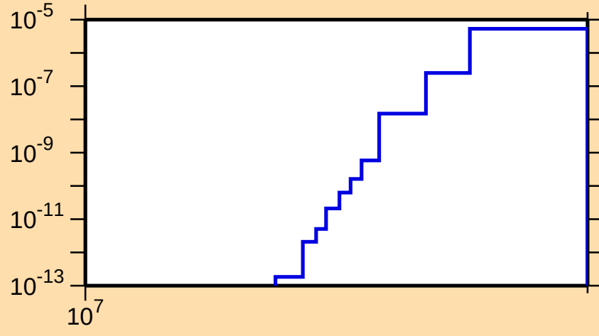
\sigma vs. E for ^{224}\text{Po}(n,nt)
