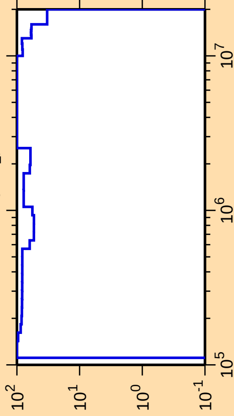
\Delta\sigma/\sigma vs. E for ^{224}\text{Po}(n,n_1)
